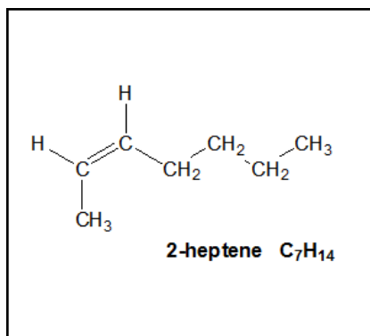
(c) Olefins
