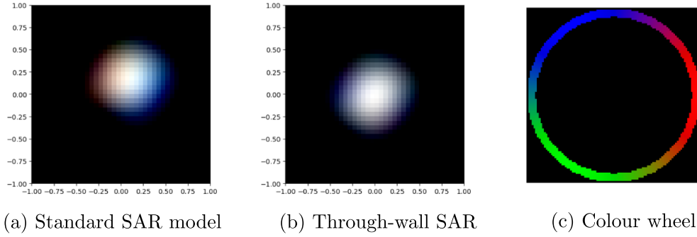
Figure 4. Overlaid magnitude of back-projection images for a single point target at the origin behind a corner wall. A separate image is formed from data of each bi-static pair in the multi-static collection. These are coloured and overlaid such that pixels taking the same value in each image which appear grey-scale, or otherwise tinted towards red, green or blue if the image is brighter in the corresponding image. Red, green and blue image colour channels also correspond to the antenna flight paths shown in figure 1.
