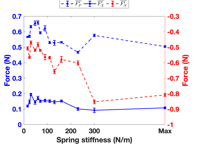
FIG. 4. Statistic analysis of pitch stiffness (Case 1 to 13).
