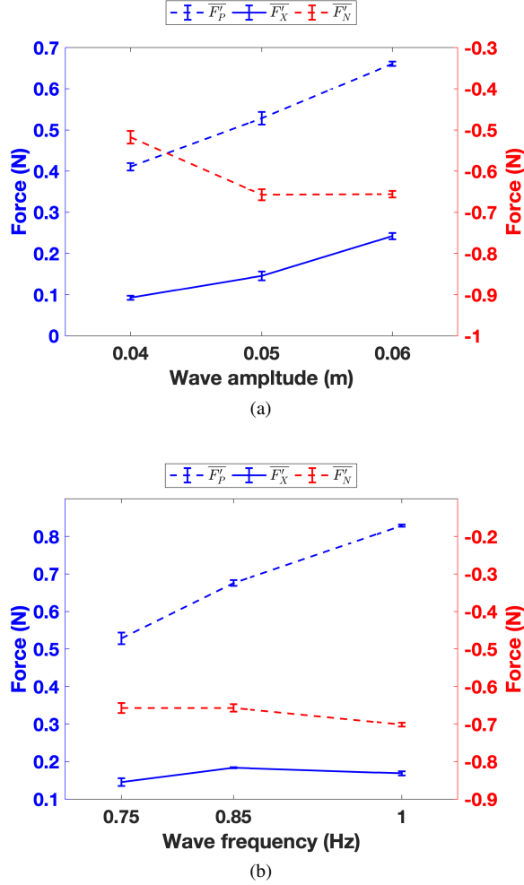
FIG. 9. Variation of \overline{F}_P' , \overline{F}_X' , \overline{F}_N' at diverse wave conditions. (a): A_W = 0.04 m, 0.05 m, 0.06 m, f_W = 0.75 Hz; (b): f_W = 0.75 Hz, 0.85 Hz, 1 Hz, A_W = 0.05 m.
