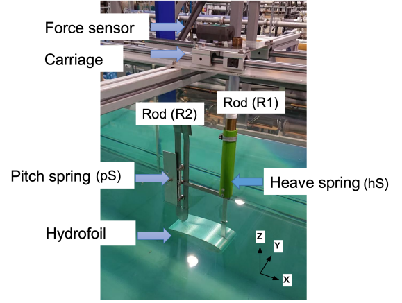
FIG. 2. Schematic sketch of experimental setup.
