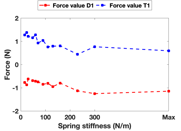
FIG. 7. Thrust peak (T1) and drag peak (D1) variation against pitch stiffness (Case 1 to 13).
