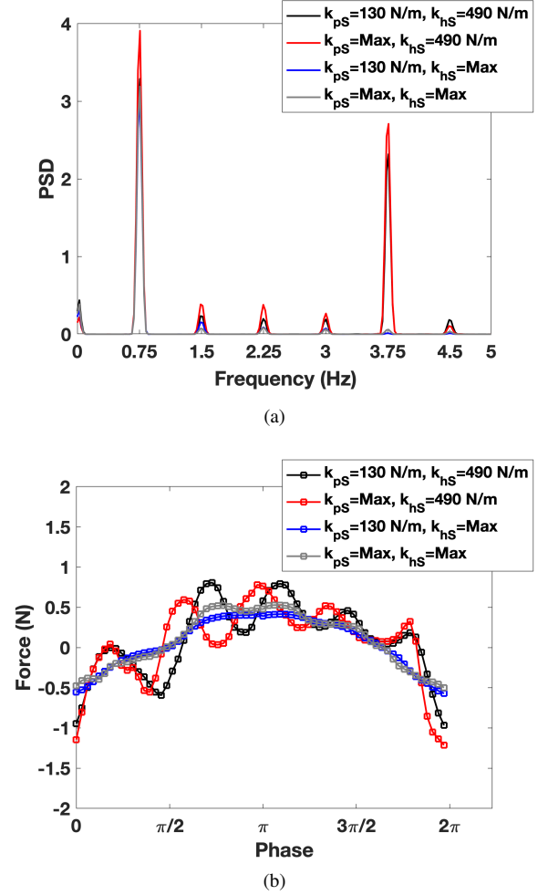
FIG. 8. Impact of number of spring-dominated DoF (Case 9, 13, 14, 15): (a) spectral analysis, (b) force variation.
