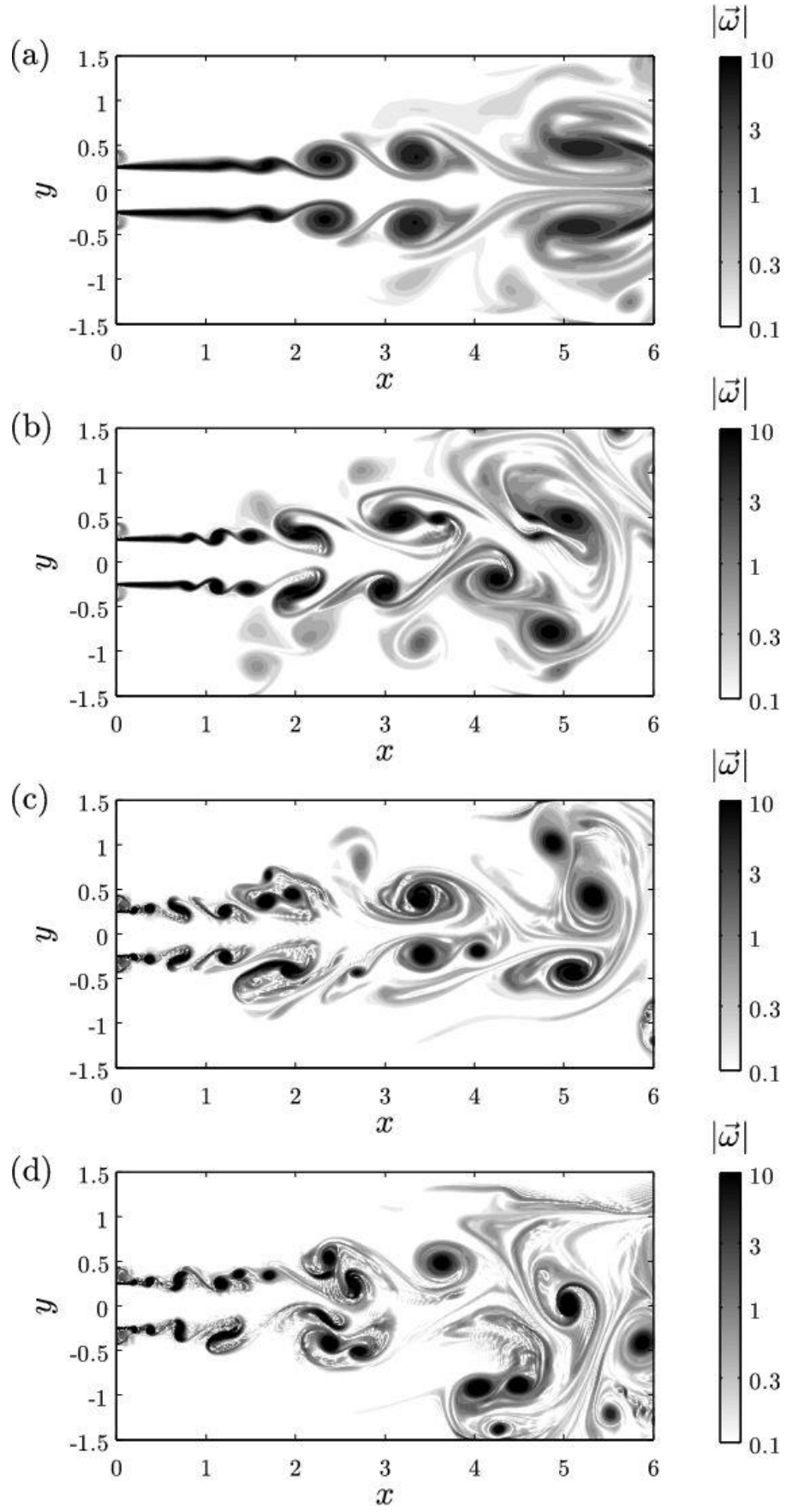
Figure 1 - Instant vorticity contours: (a) \text{Re} = 5000 ; (b) \text{Re} = 10,000 ; (c) \text{Re} = 20,000 ; (d) \text{Re} = 40,000 .
