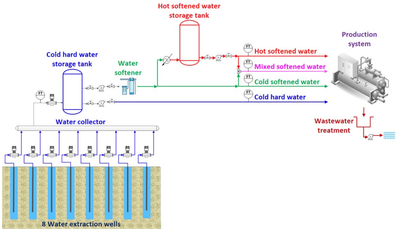
Figure 5. A schematic representation of the hydraulic circuit and water-monitoring system.
