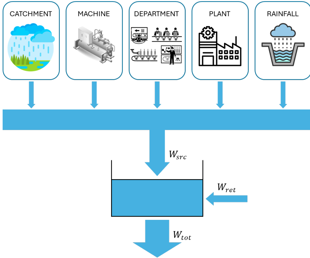
Figure 2. Possible streams within the virtual water source.
