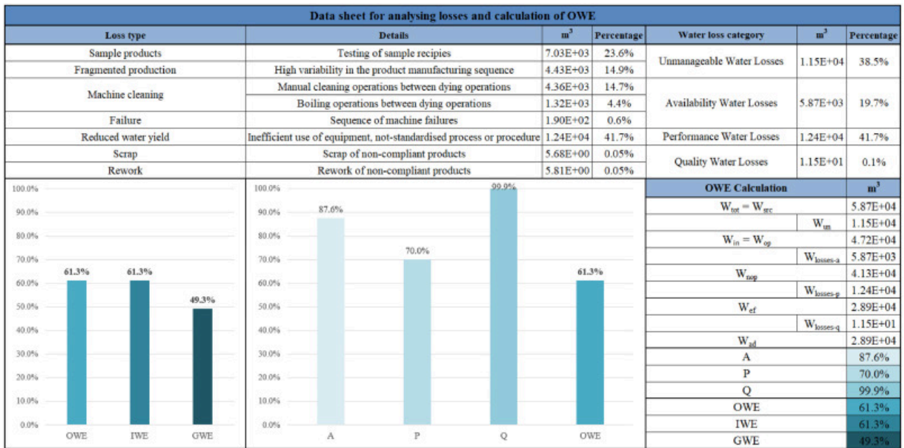
Figure 6. Datasheet for OWE calculation.
