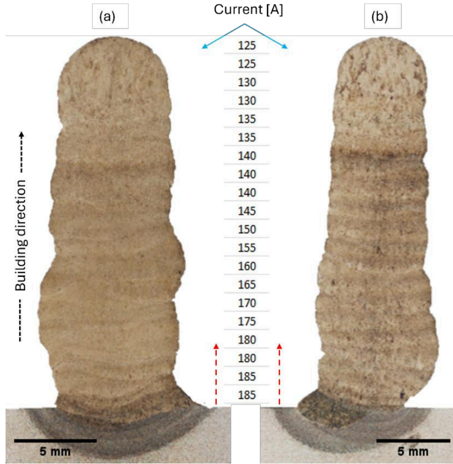
Fig. 9 Deposition strategy for thin walls in PTA-WAAM, employing (a) cored-wire, and (b) solid wire
