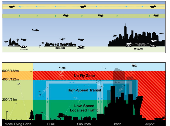
Fig. 1. Airspace structures proposed by the FAA [1] (top) and Amazon [14] (bottom).
