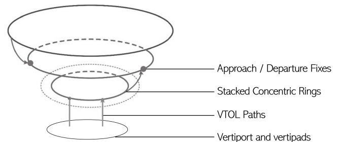
Fig. 3. Generic ring-based proposal to structure vertiport airspace.
