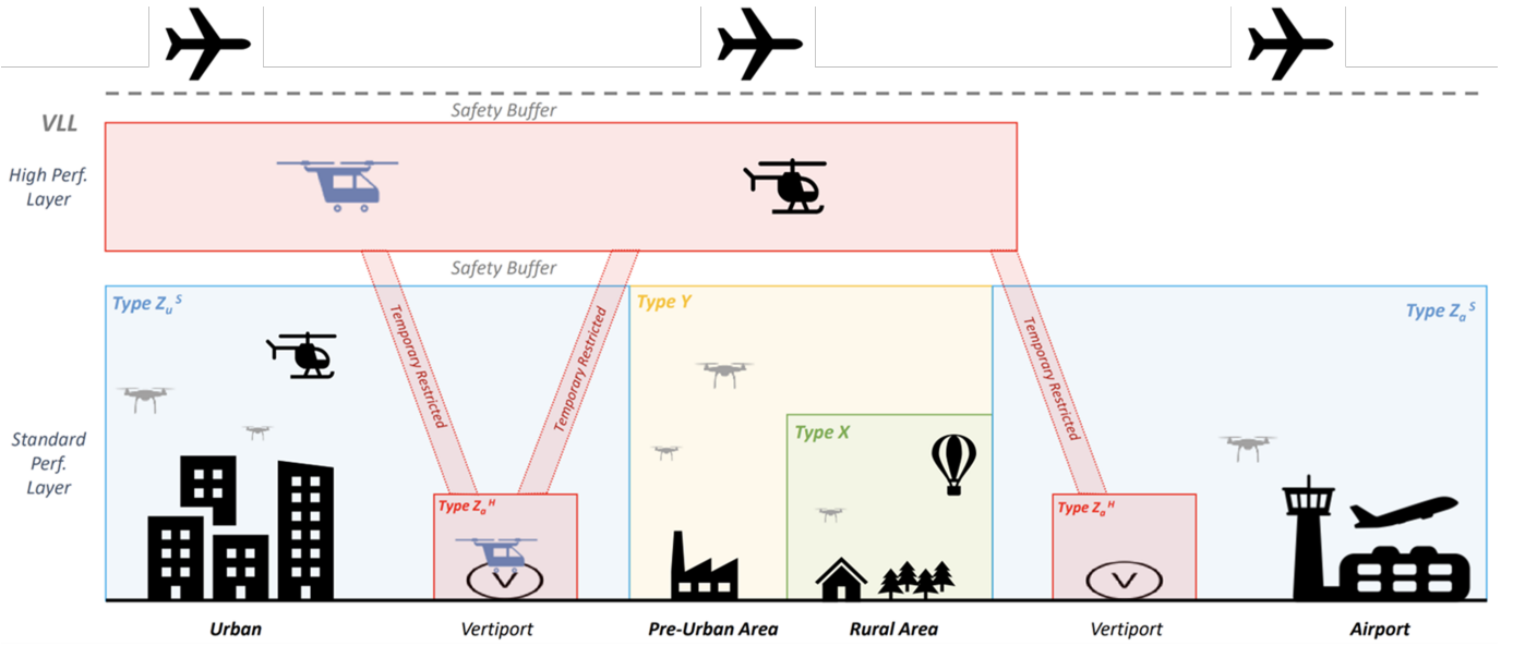
Fig. 2. Layered airspace structure proposed in AMU-LED, including dynamic corridors for vertiport take-offs and landings [16].
