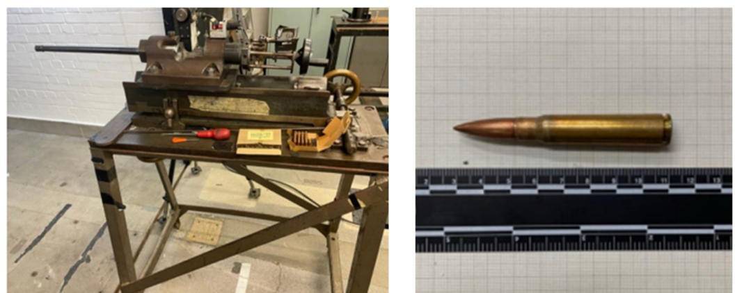
Figure 1. LEFT: Image of No.3 proof mount with Mauser barrel rifle. RIGHT: Image of 7.92 \times 57 mm Mauser ammunition [23].
