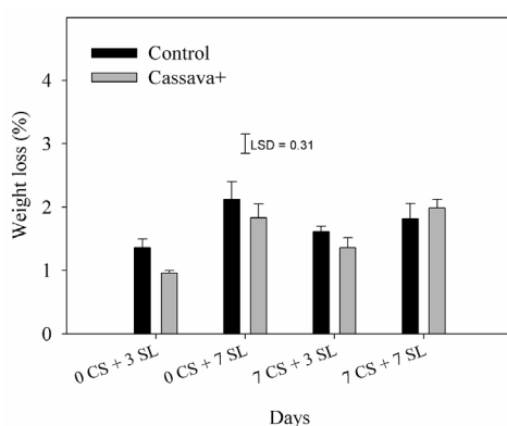
Figure 2. Weight loss (%) of coated (Cassava+) and uncoated (Control) asparagus spears, with previous cold storage for seven days (7CS) at 1 °C and 90% RH, or without cold storage (0CS), followed by 3 (3SL) or 7 (7SL) days of shelf-life condition at 7 °C and 70% RH.
