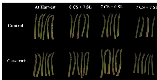
Figure 1. Appearance of uncoated (control) and coated (Cassava+) asparagus spears at harvest, with previous cold storage for seven days (7CS) at 1 °C and 90% RH, or without cold storage (0CS), followed by zero (0SL) or 7 days (7SL) of shelf-life condition at 7 °C and 70% RH.
