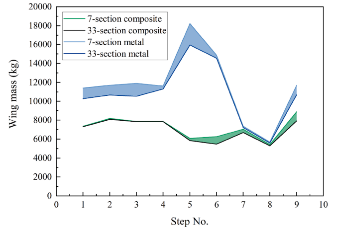
Fig. 10. Comparison of wing mass predictions from 7-section and 33-section models for composite and metallic wings across the sensitivity-analysis steps.
