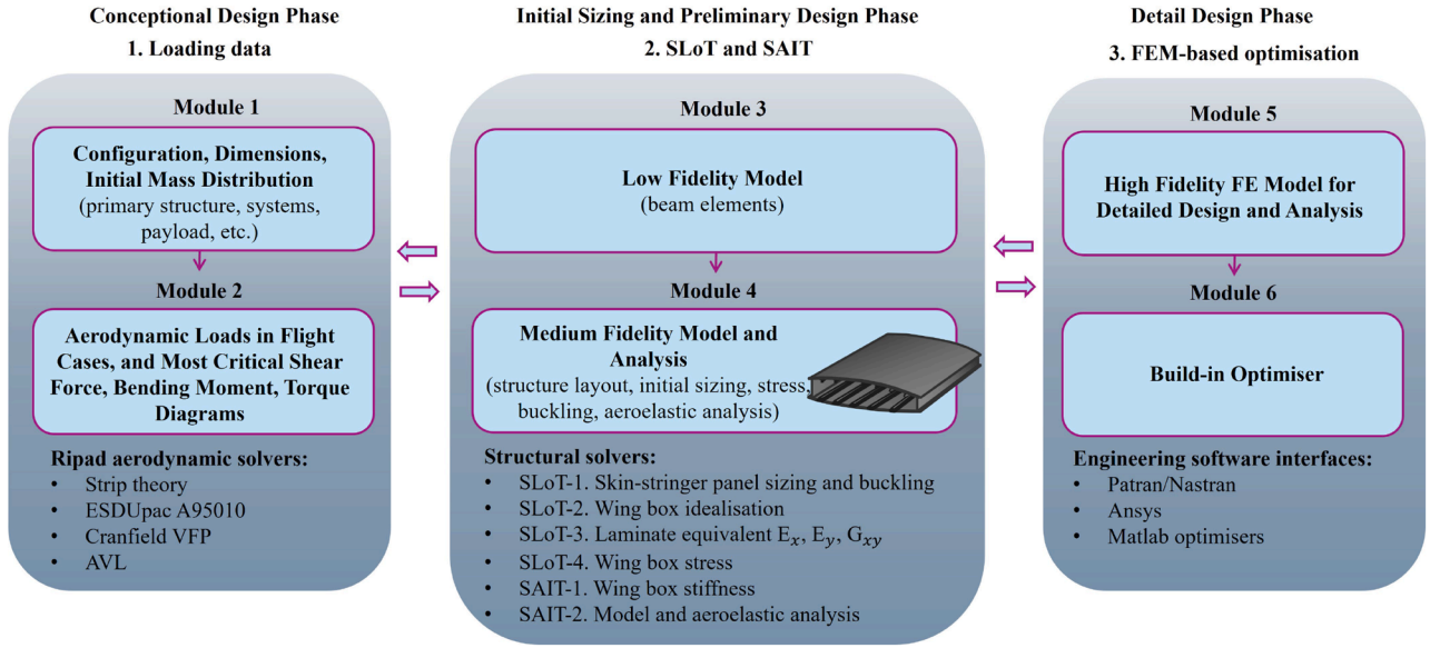
Fig. 1. Overview of a flexible multi-fidelity toolset across three design phases.
