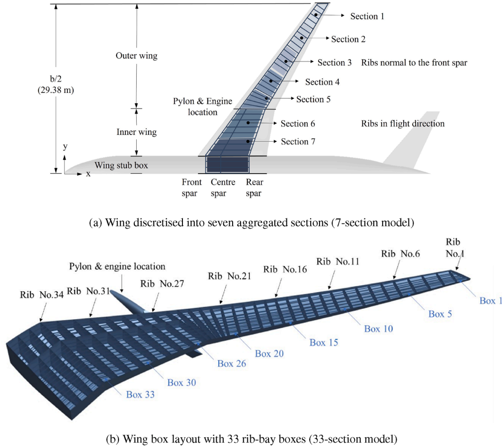
Fig. 3. Wing-box structural layout and discretisation.
