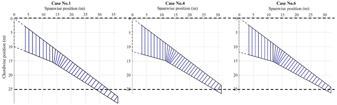
Fig. 14. Wing planform and rib layouts of Cases 1, 4, and 6.
