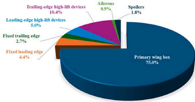
Fig. 4. Mass breakdown of the wing structure.
