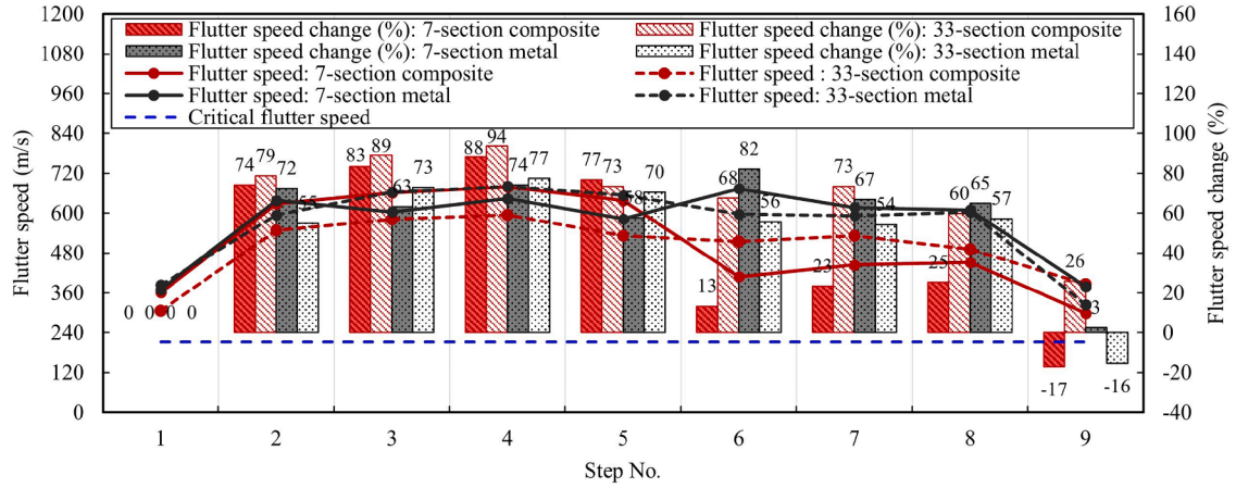
Fig. 13. Flutter speed at sea level with percentage changes for each model across the sensitivity analysis steps.
