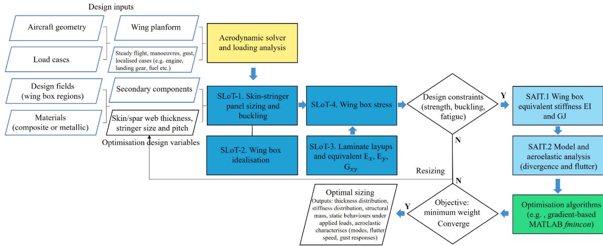
Fig. 2. MDO sizing workflow.
