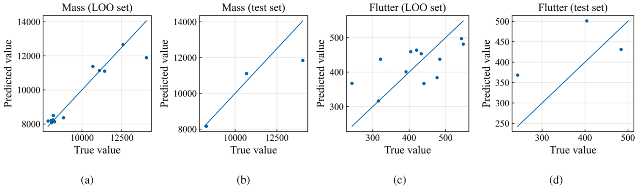
Fig. 15. Parity plots of RF predictions for wing mass (kg) and flutter speed (m/s).
