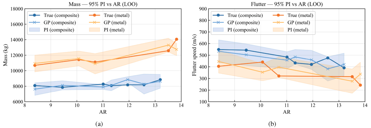
Fig. 17. GPR LOO predictions and 95% prediction intervals versus AR for (a) mass and (b) flutter speed, comparing composite and metallic wings.
