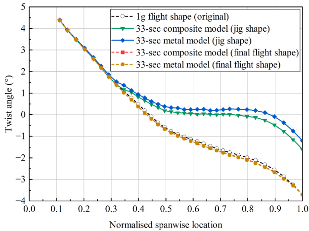
Fig. 9. Estimated jig shapes and 1-g flight shapes of the sized wings, compared with the CRM design flight shape.
