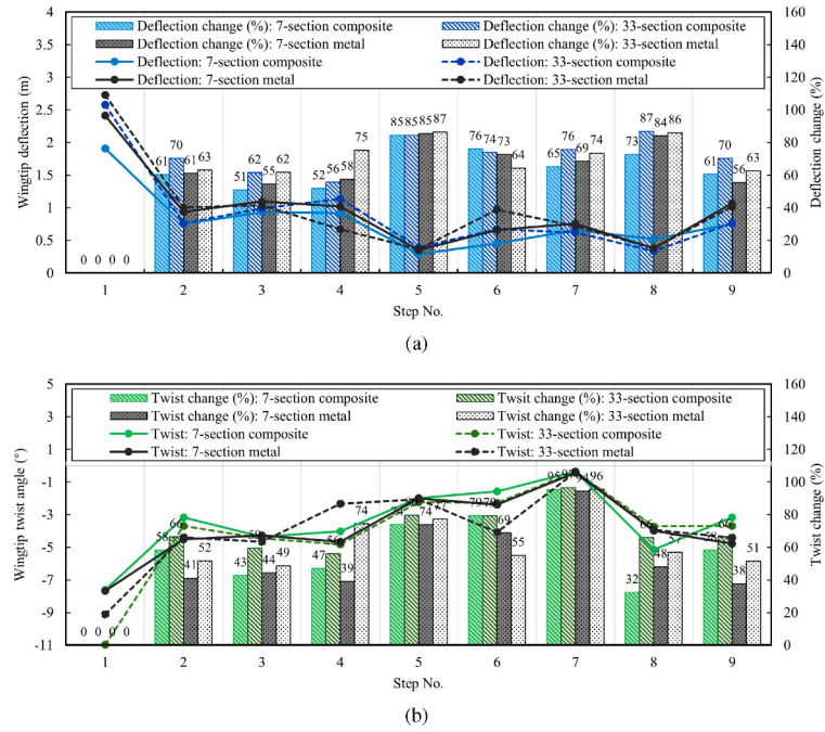
Fig. 12. (a) Wingtip deflection and (b) twist angle with percentage changes across the sensitivity analysis steps.
