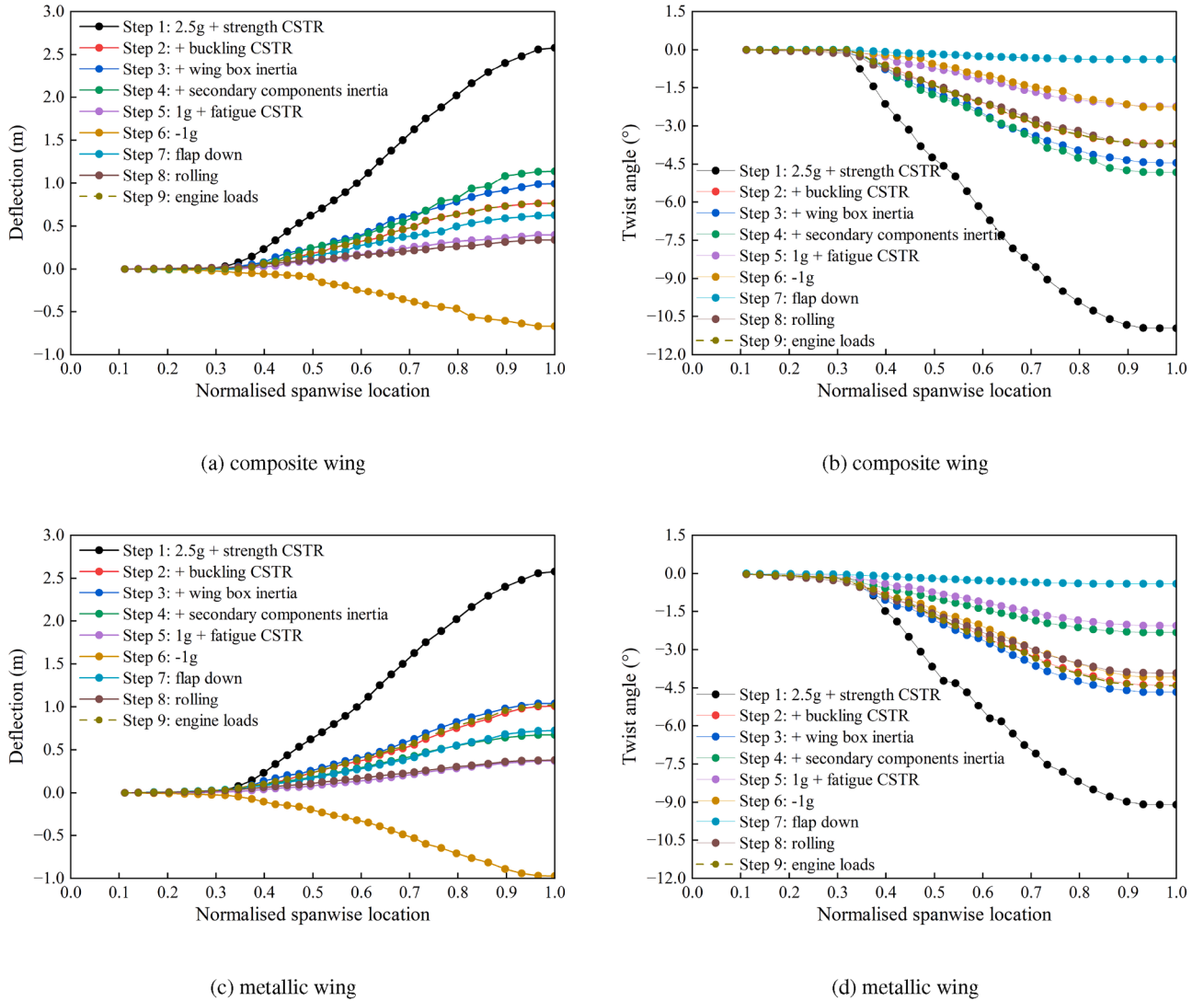
Fig. 11. Spanwise distributions of structural behaviour for the 33-section model across all steps of the sensitivity analysis: (a) deflection and (b) twist angle of the composite wing; (c) deflection and (d) twist angle of the metallic wing.
