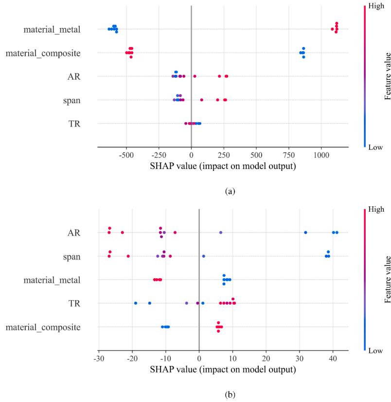
Fig. 16. Global SHAP summary for (a) mass and (b) flutter speed.
