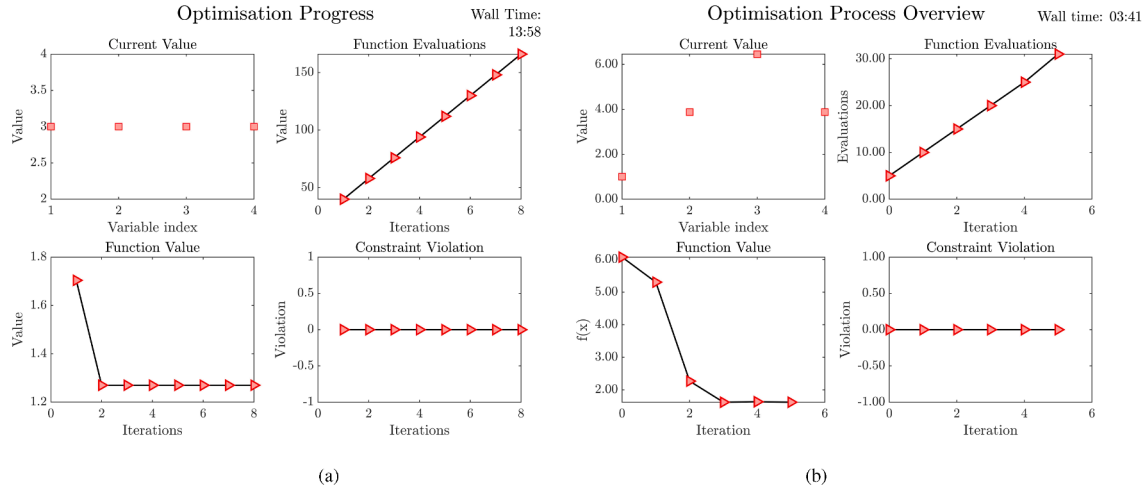
Fig. 6. Sizing optimisation process for a single-cell (a) composite wing box and (b) metallic wing box.
