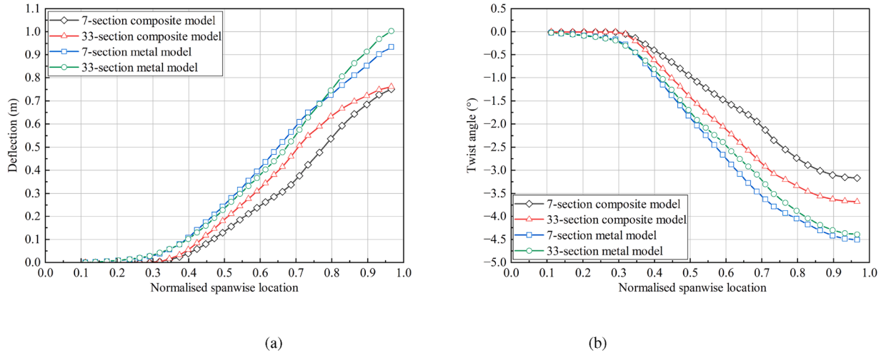
Fig. 8. (a) Spanwise deflection and (b) elastic twist of the sized wings with variable stringer pitch under the 2.5-g load.
