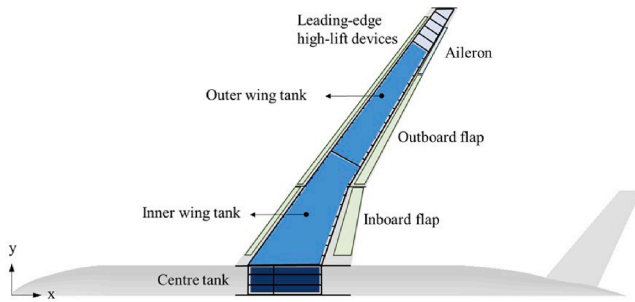
Fig. 5. Schematic layout of secondary structures and fuel tanks.
