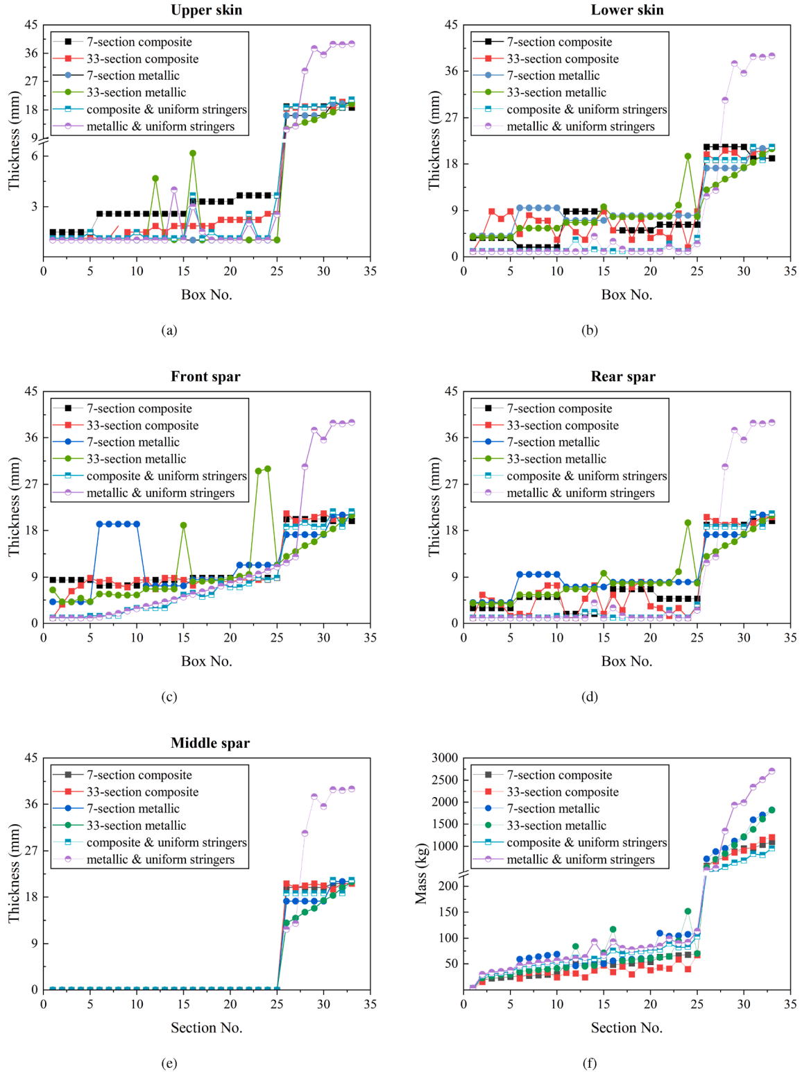
Fig. 7. Spanwise sizing results for composite and metallic wings obtained using coarse 7-section and refined 33-section models under the 2.5-g load case.
