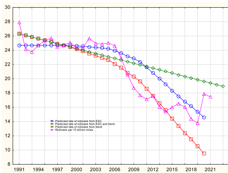
Fig. 4. Predicted and actual trend for fatal rollovers per 10 billion miles in the US.
