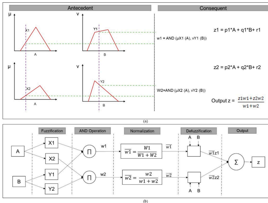
Figure 7. (a) First order Takagi–Sugeno fuzzy reasoning (b) Adaptive Neuro-Fuzzy Inference System (ANFIS) structure (adapted from [30]).
