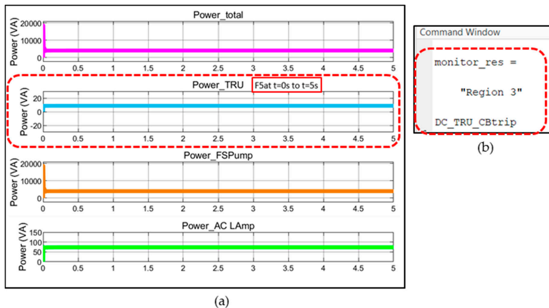
Figure 14. (a) Corresponding reaction in apparent power for DC TRU_CBtrip (F5) fault injection. (b) Method 2 results with the ANFIS monitor and causal reasoning.
