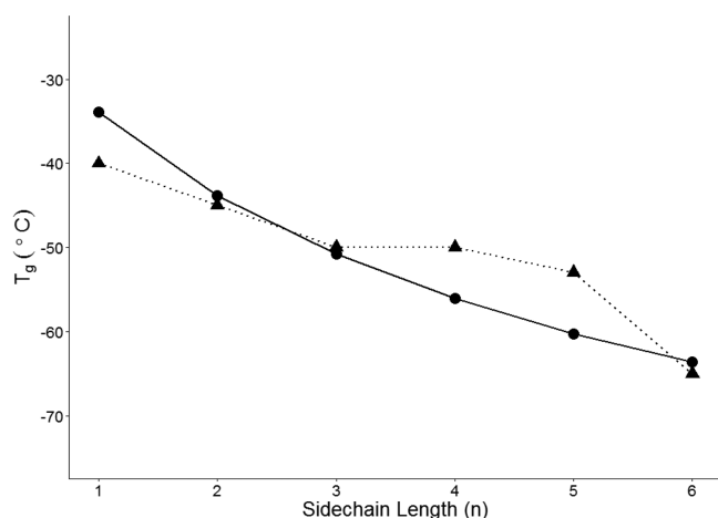
Figure 4. T_g values for polyolefins with varying side chain lengths; n is the number of carbon atoms in the side chain. GIM predicted (solid line, dots) and experimental data (dashed line, triangles) from the literature.
