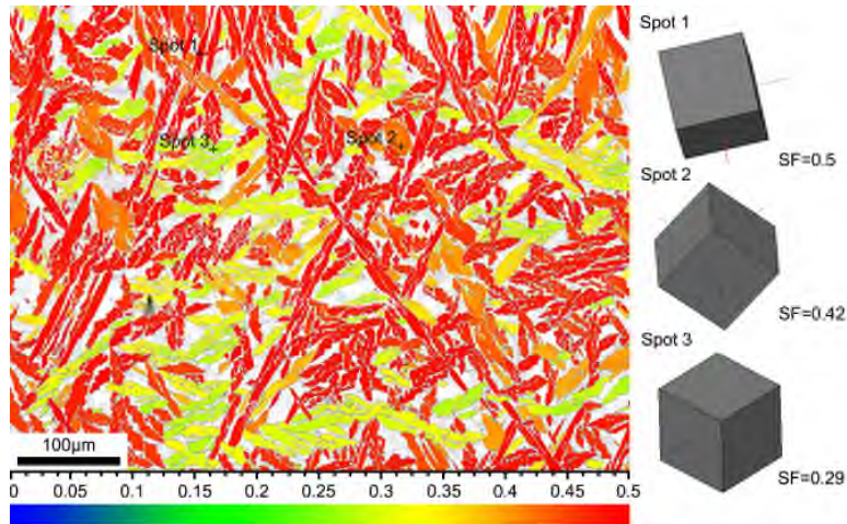
Fig. 18 SF distribution of the austenite phase in the wall-body area under the following assumption: 1), the active slip system is [111]\langle\bar{1}10\rangle ; 2), the applied stress direction is parallel to the X direction.
