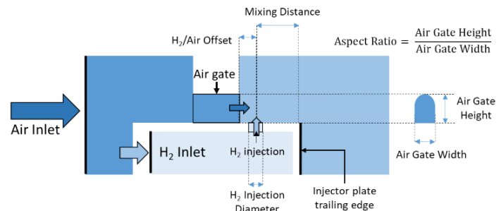
Figure 1. H 2 micromix single injector design parameters
