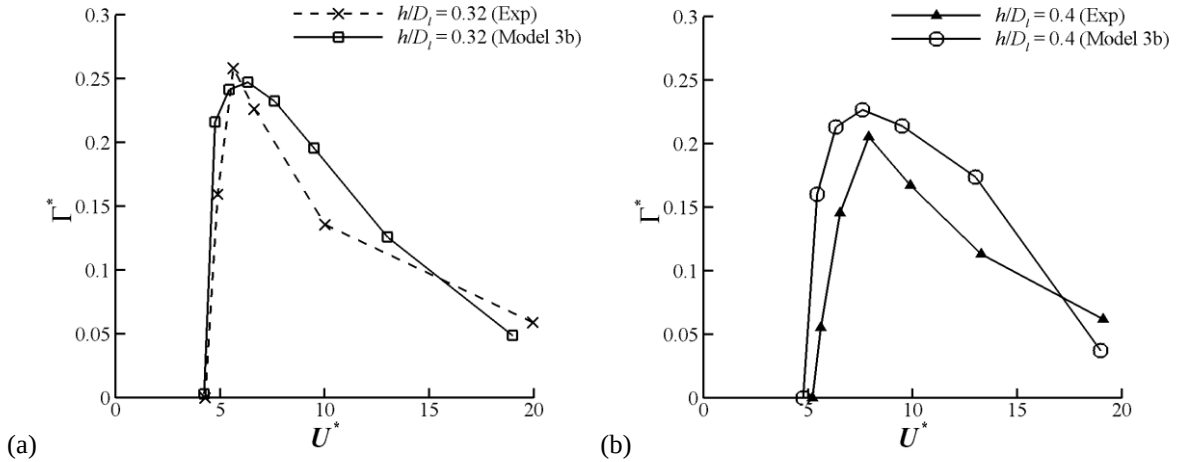
Fig. 14: Predicted total non-dimensional vortex strength against velocity ratio with the empirical constant applied for (a) h/D_l = 0.32 , and (b) h/D_l = 0.40 with \delta^*/D_l = 0.11 , M_i = 0.58
