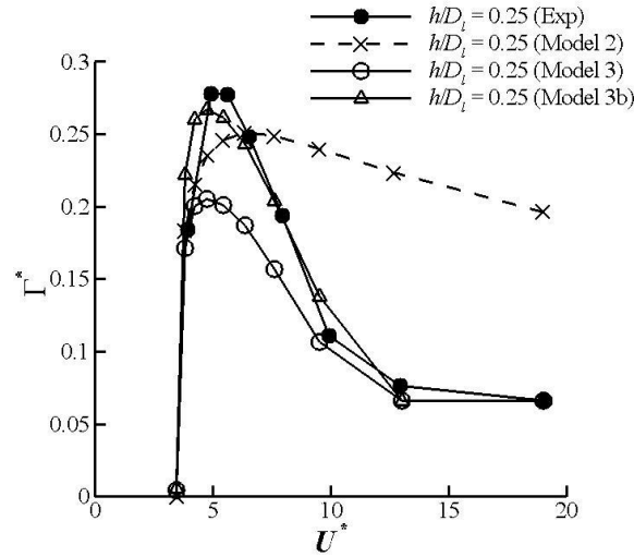
Fig. 13: Predicted non-dimensional vortex strength against velocity ratio for Model 3 with comparison to Model 2 and the experimental results ( h/D_l = 0.25 , \delta^*/D_l = 0.11 , M_l = 0.58 )
