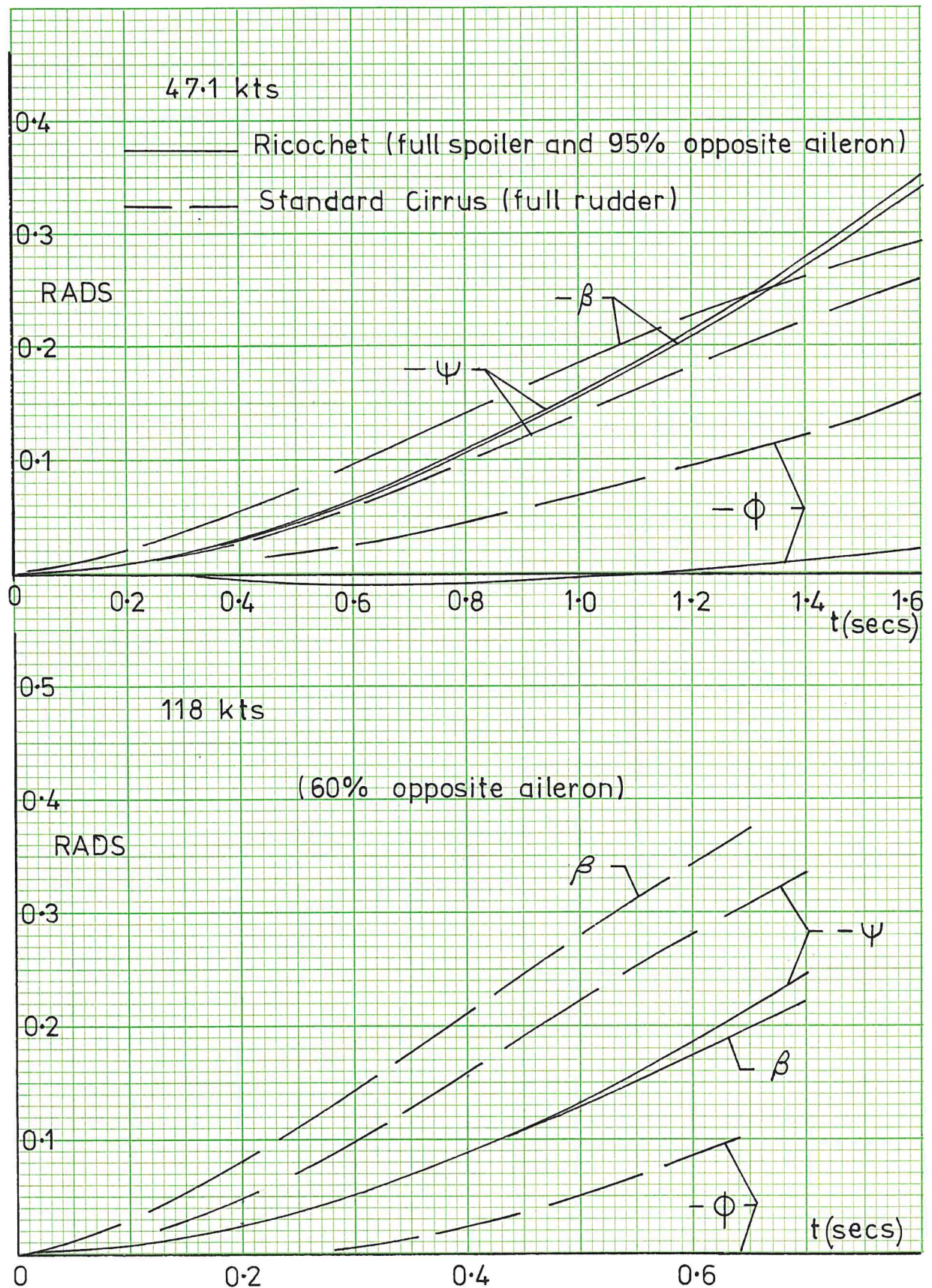
FIG 34 RESPONSE DUE TO INSTANTANEOUS APPLICATION OF FULL SPOILER AND PART DEFLECTION OF OPPOSITE AILERON, NO WATER BALLAST
