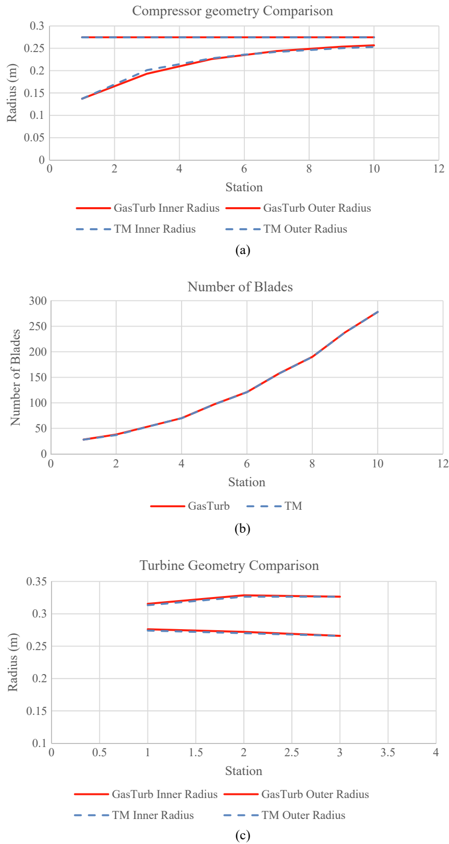
Fig. 13. Geometry comparison between TM and GasTurb.
