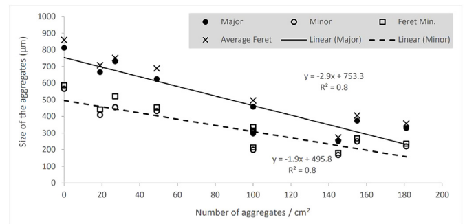
Fig. 9. The sizes of aggregates in the various PVC – aggregate composite surfaces in different measuring directions.
