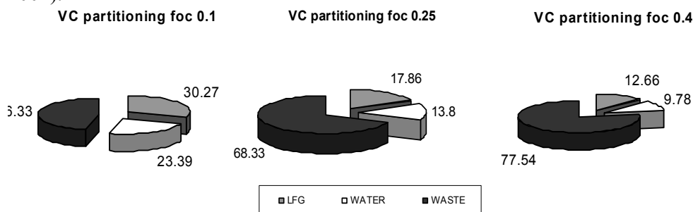
Figure 3. Illustrative mass contributions (% w/w ) of vinyl chloride (VC) to LFG, water and waste phases contingent on the fraction of organic carbon ( f_{oc} ) in the system
