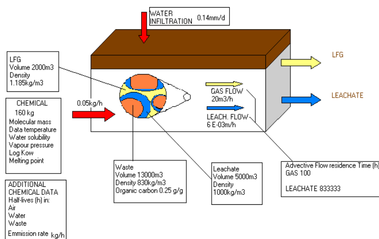
Figure 2. Evaluative environment for Level II model
