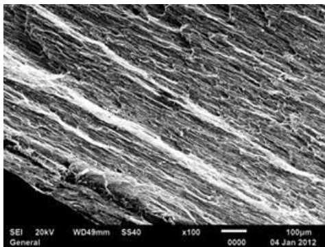
(b) Base region: V_i = 680 m/s (SEM 100 x mag.)
