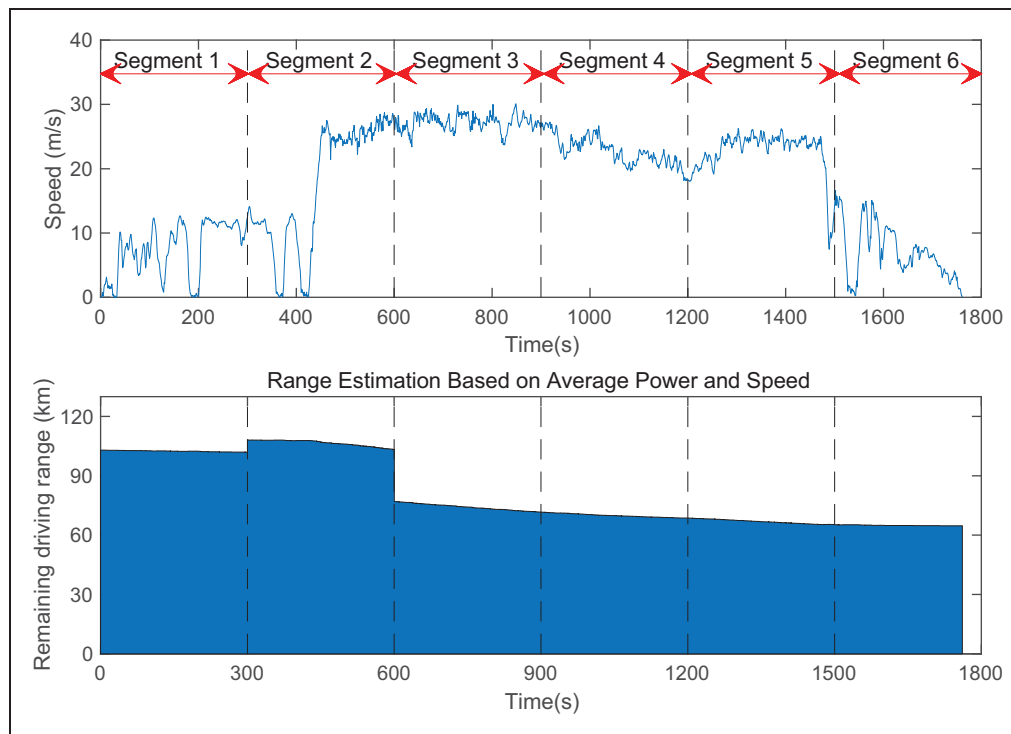
Figure 21. RDR estimation during Test 3 based on average power and average speed.
