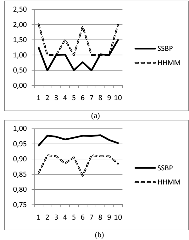
Fig. 11. Comparison of SSBP and HHMM using a) RMSE b) R-square
