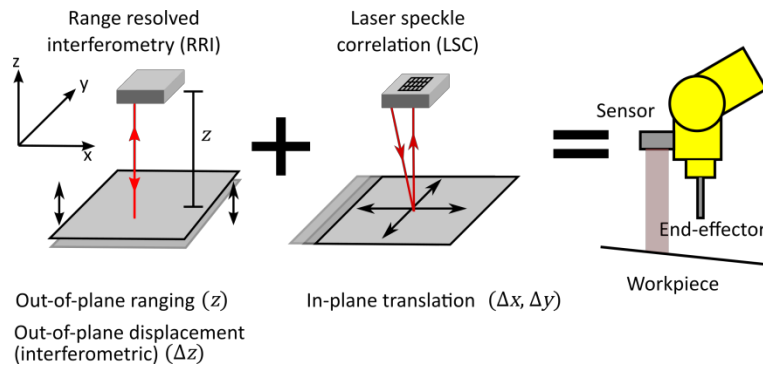
Figure 1. Operating concept of the wPOS instrument combining Range Resolved Interferometry (RRI) and Laser Speckle Correlation sensing (LSC)
