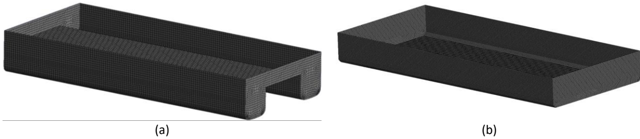
Fig. 4. Mesh visualization: (a) Twin hull (b) Monohull
