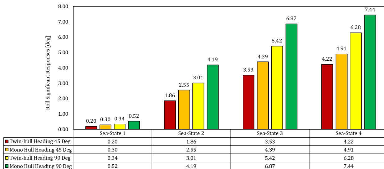
Fig. 15. Roll significant responses
