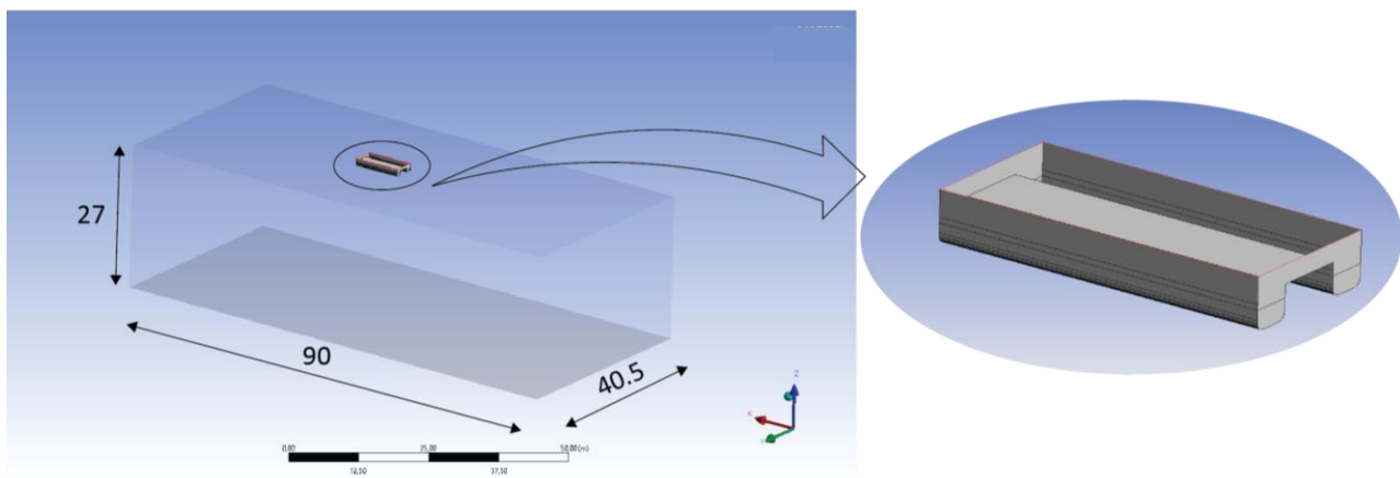
Fig. 3. Computational domain in Ansys Aqwa. Unit in meter
