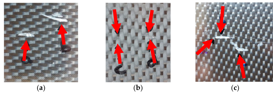
Figure 15. Images of damages on the (a) front face and (b) back face of panel 1 and on the (c) front face of panel 3.
