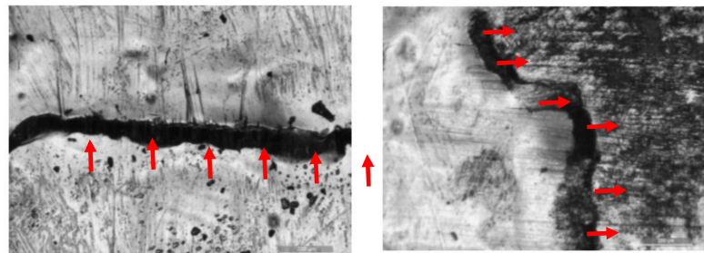
Figure 6. Optical images of the front faces of panels 13 ( left-hand side ) and 15 ( right-hand side ) detailing the matrix cracks perpendicular to the fibre direction (crack highlighted with red arrows).
