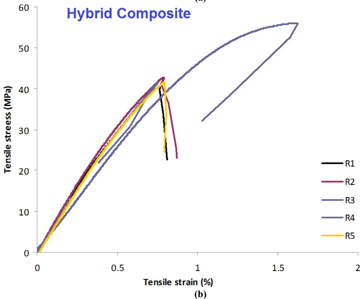
Figure 7 Tensile stress versus strain of (a) PLA, (b) hybrid composites
