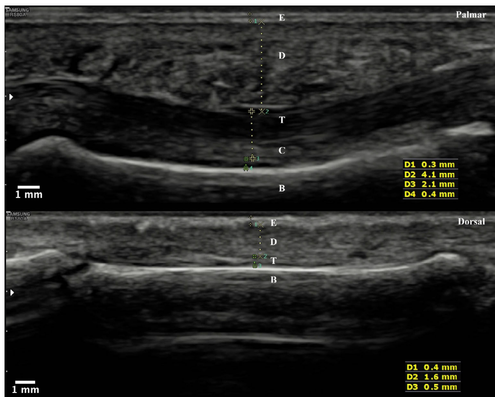
FIGURE 1 Longitudinal orientation of the probe allowed imaging along the length of the finger, quantifying the anatomical entities. The layers are measured are epidermis (denoted as E, with D1 being the measurement), dermis (D, D2), tendon (T, D3), connective tissue (C, D4) and the bone (B). Both the palmar and dorsal sides of the finger are measured to complete the finger structure
