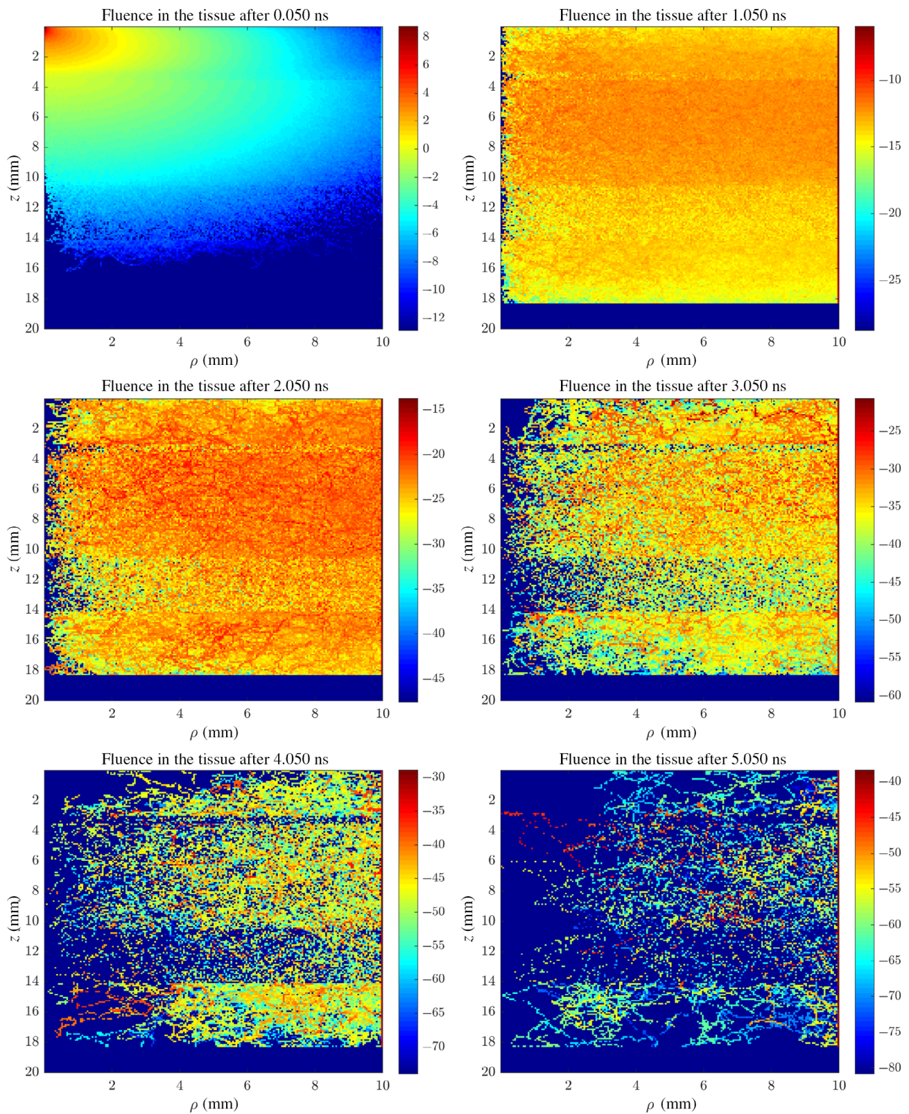
FIGURE 7 The fluence of the photons at 830 nm wavelength in the tissue volume ( \text{mW}/\text{mm}^{-3} ) as a function of cylindrical coordinates ( \rho : mm) and depth ( z ) is illustrated at different instances after emission from the sources for the optical model for participant USP005 (Table 1)
