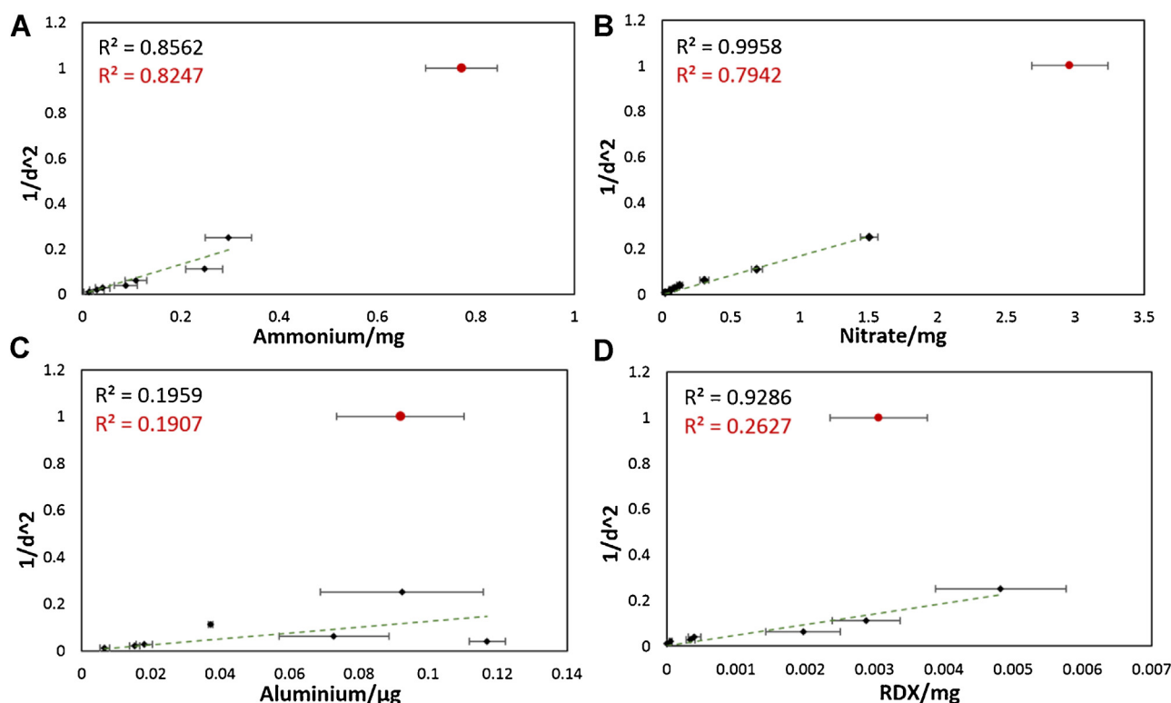
Fig. 2. Total amount of explosive residue detected at each sampled distance compared to ' 1/d^2 ' representing the inverse-square law model, where d is the distance from between 1 and 10 m. Data from the 1 m sampling points is included as a red point and R^2 values for linearity both with the 1 m datum (in red) and without (in black) are inset. Error bars indicate standard deviation of measurements over 6 repeat firings. (For interpretation of the references to colour in this figure legend, the reader is referred to the web version of this article.)
