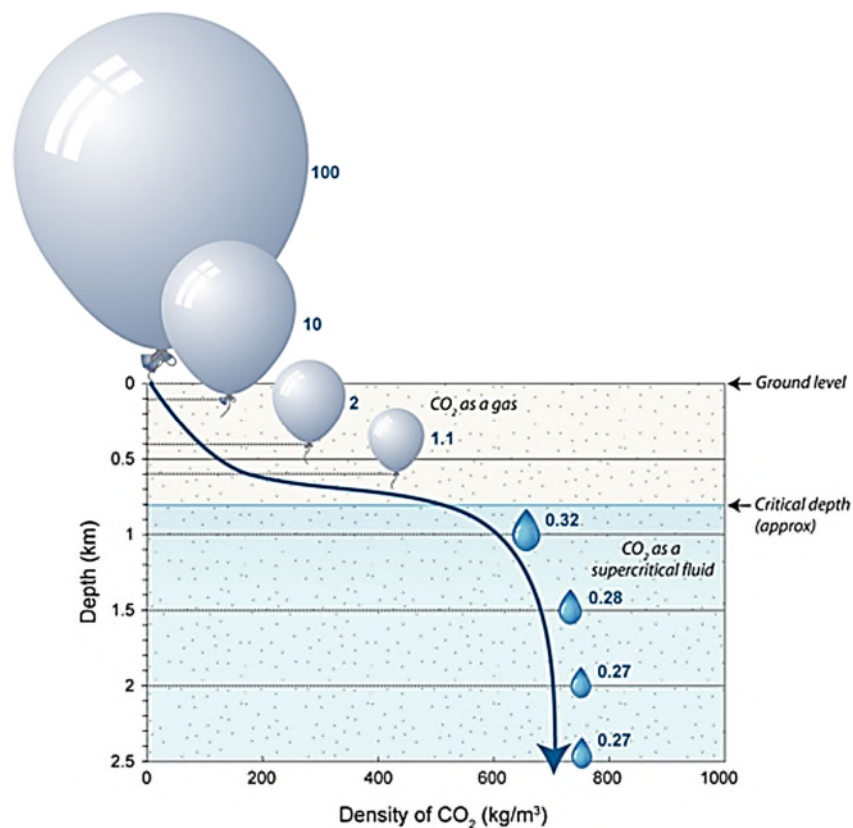
Figure 4: Relative volumes of \text{CO}_2 stored underground as a function of depth in storage reservoirs [162]. Note: Blue numbers in this figure represent relative volume of \text{CO}_2 at each depth.
