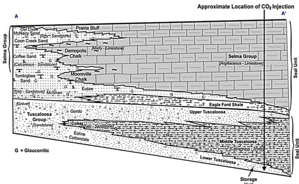
Figure 18: Cross section (AA') of lithofacies within the Cranfield Project with approximate location of CO 2 injection. (reprinted with permission from Griffith et al. [296], Copyright 2017, Springer).
