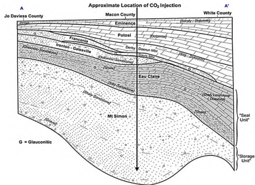
Figure 19: Cross section (AA') of lithofacies within the Decatur Project with approximate location of CO 2 injection showing the Mt. Simon formation as storage unit and the overlying Eau Claire formation as seal unit (reprinted with permission from Griffith et al. [296], Copyright 2017, Springer).
