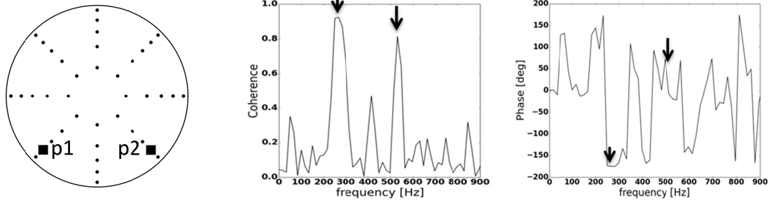
Figure 11 Coherence and phase distribution between two opposite points on the AIP. S-Duct 2A.
