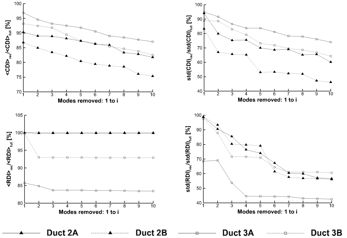
Fig. 18 Spectral distribution of the total pressure POD coefficients.
