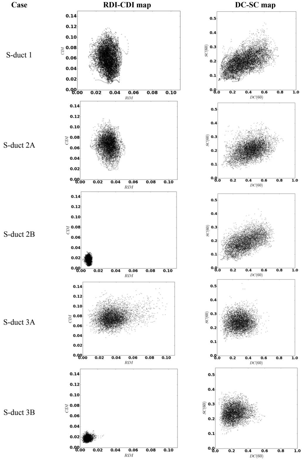
Figure 9 Distortion metric maps from DDES temporal snapshots at the AIP section
