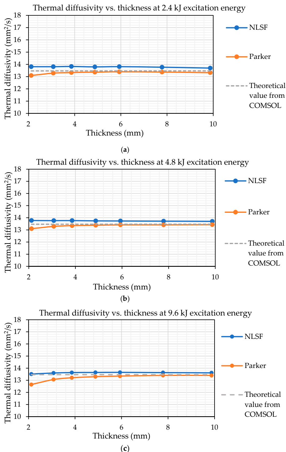
Figure 4. Thermal diffusivity measurements using the NLSF algorithm and Parker’s method for a 150 × 100 mm S275 steel plate with multiple thicknesses, subjected to different energy levels of pulsed heating simulated in COMSOL. Thermal diffusivity estimates at (a) 2.4kJ (b) 4.8kJ and (c) 9.6kJ.
