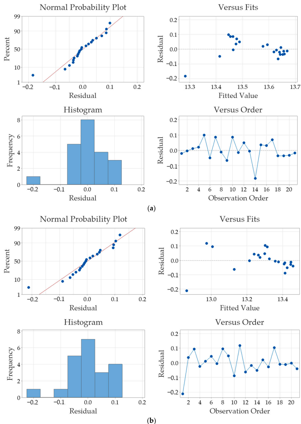
Figure 9. Residual plots from the finite element simulations for estimating thermal diffusivity using (a) NLSF and (b) Parker's method.
