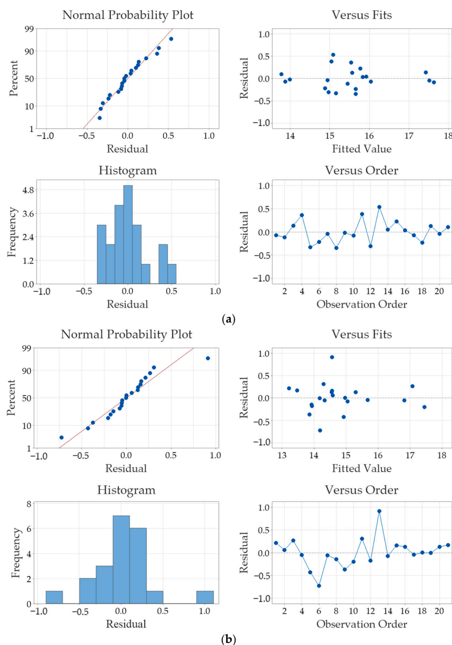
Figure 16. Residual plots from laboratory experiments for estimating thermal diffusivity using (a) NLSF and (b) Parker.
