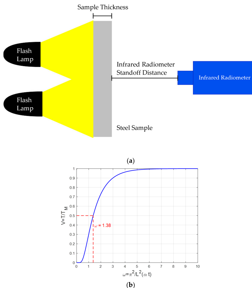
Figure 1. (a) Illustration of the PT transmission mode configuration; (b) nondimensionalised back wall temperature plot displaying the value for \omega at half the maximum temperature.
