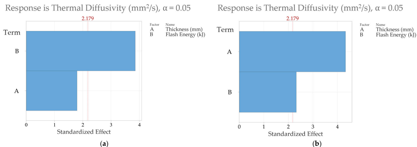
Figure 8. Pareto charts for standardised effects for the finite element simulations (a) thermal diffusivity estimated using NLSF and (b) thermal diffusivity estimated using Parker's method.
