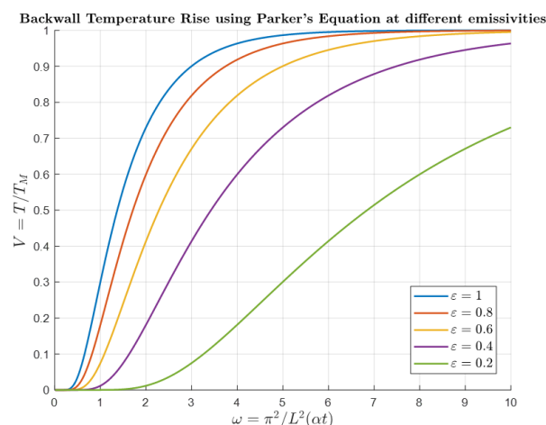
Figure 2. Normalised back wall temperature profile at different emissivity values.
