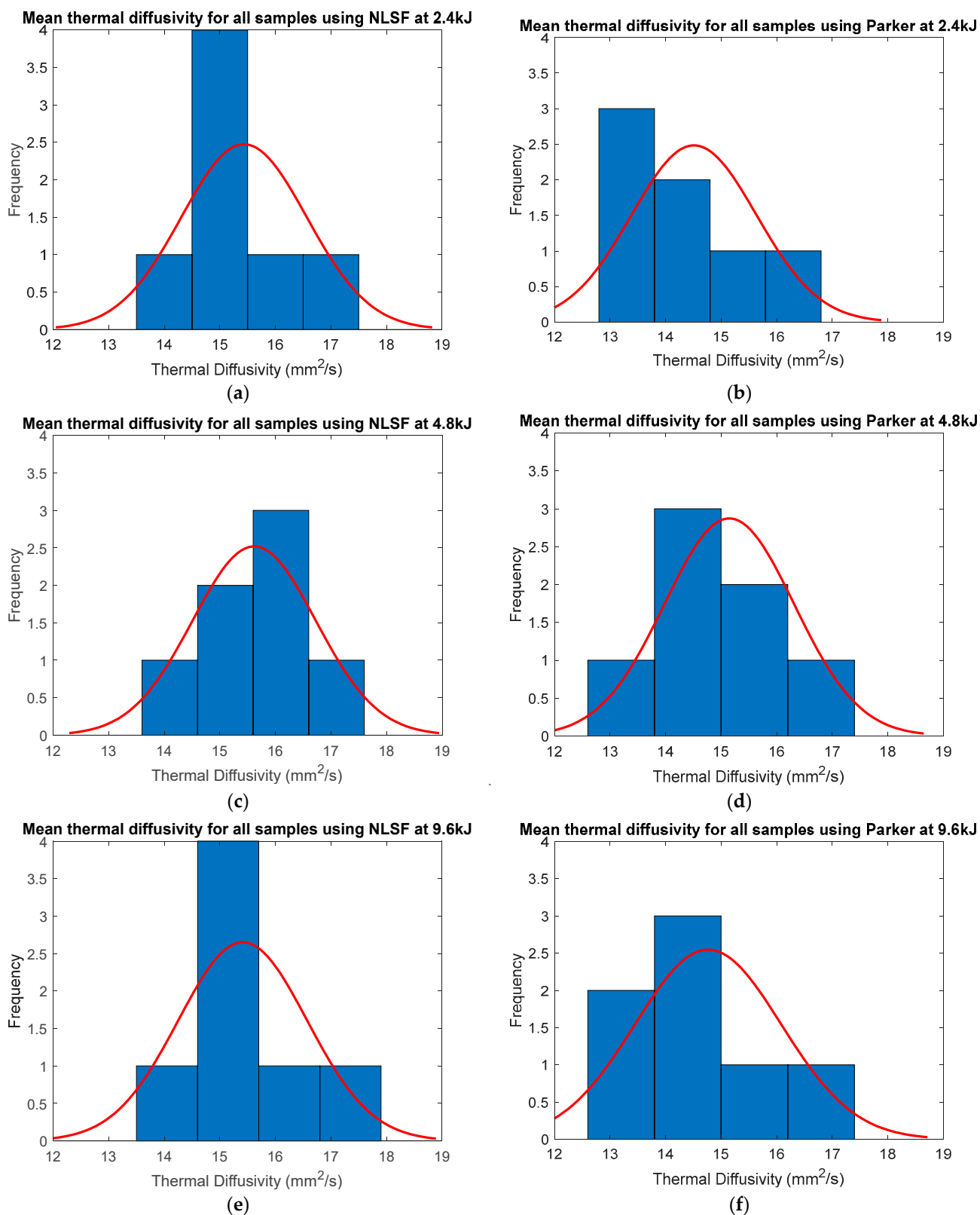
Figure 12. Histograms showcasing variations in thermal diffusivity with different thicknesses at different energy levels estimated using NLSF (a,c,e) and Parker's methods (b,d,f).
