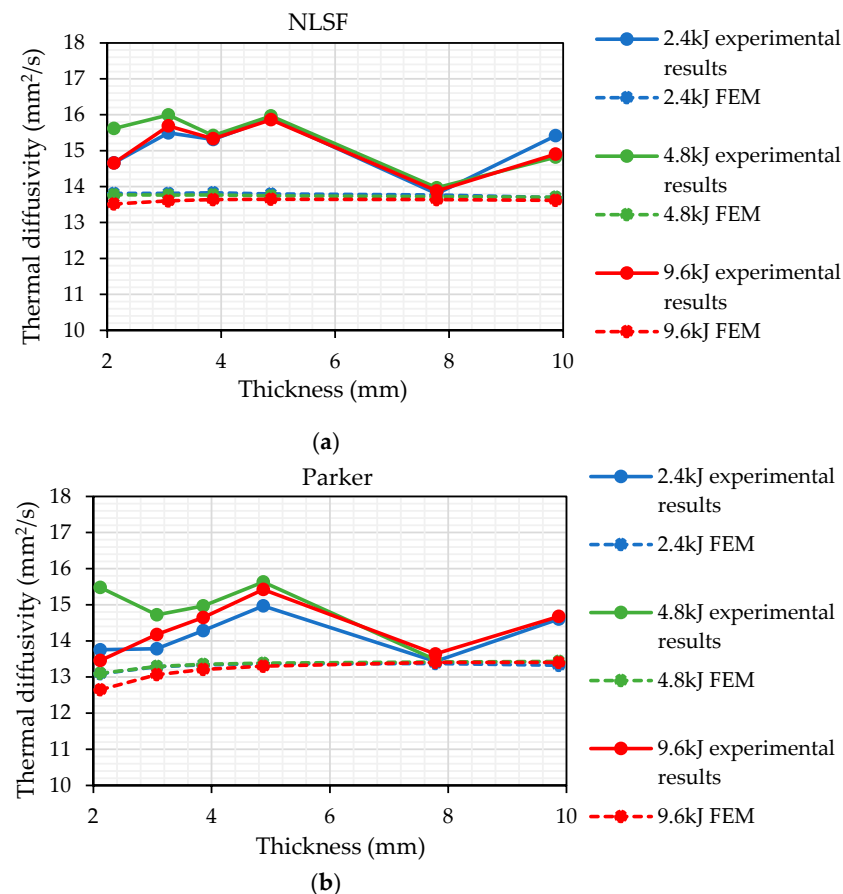
Figure 15. Comparison between simulation and laboratory experiments for thermal diffusivity measurement (a) using the NLSF method and (b) using Parker's method.
