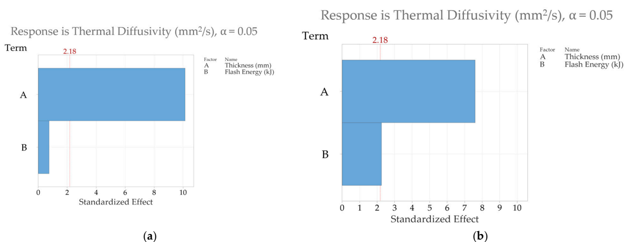
Figure 13. Pareto charts for standardised effects for the laboratory experiments (a) thermal diffusivity estimated using NLSF and (b) thermal diffusivity estimated using Parker's method.
