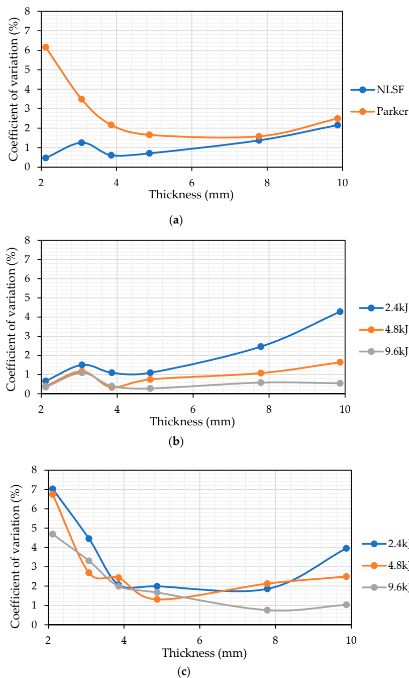
Figure 14. Comparison of the coefficient of variation (a) comparison between the NLSF and Parker methods, (b) variation at different thicknesses using the NLSF method, and (c) variation at different thicknesses using Parker's method.
