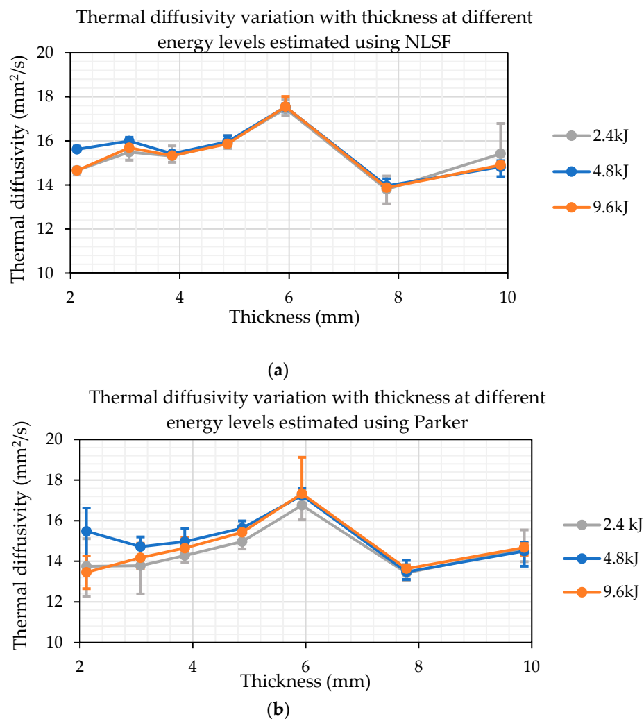
Figure 11. Thermal diffusivity measurements for varying thicknesses at different energy levels, estimated using (a) NLSF and (b) Parker's method.
