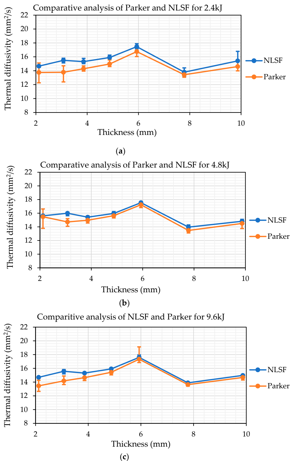
Figure 10. Thermal diffusivity estimations for different thicknesses at (a) 2.4kJ, (b) 4.8kJ, and (c) 9.6kJ using NLSF and Parker's methods.
