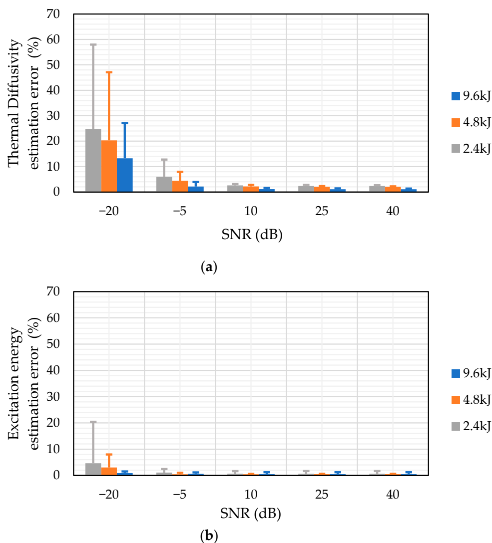
Figure 6. Error analysis of the NLSF algorithm with varying SNRS for (a) thermal diffusivity measurement and (b) input energy measurement using the temperature plots obtained from the FEA model in COMSOL.
