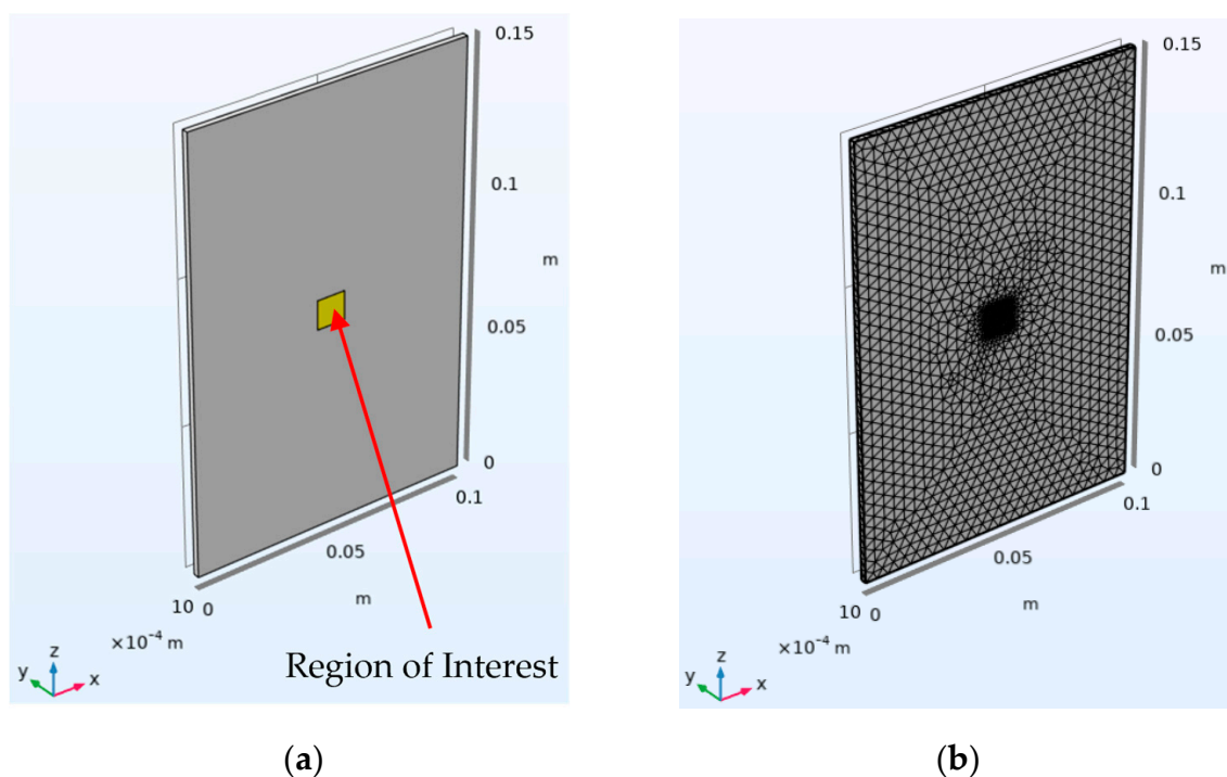
Figure 3. Geometry for the FEA Model. (a) The yellow region is where the temperature measurements are taken from at the back wall. (b) The meshed geometry is where the region of interest has a finer geometry to save computational time.
