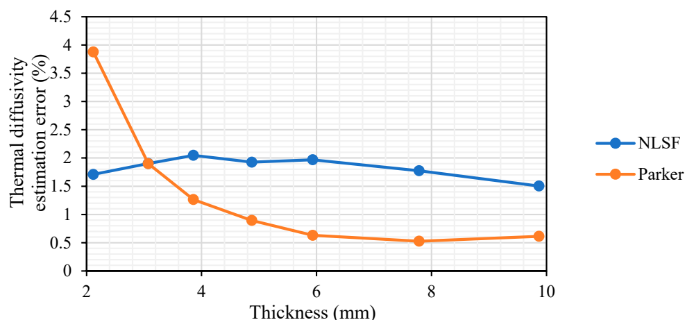
Figure 5. Measurement error for NLSF and Parker's method across all thicknesses (values have been averaged across the three different energy levels).
