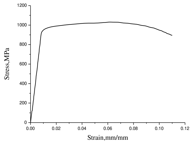
(a) Ti-6Al-4V stress-strain curve
