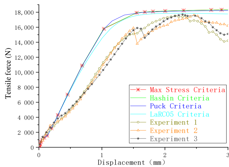
Figure 5. Force-displacement curves.
