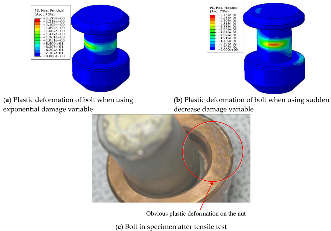
Figure 8. Plastic deformation of a bolt.
