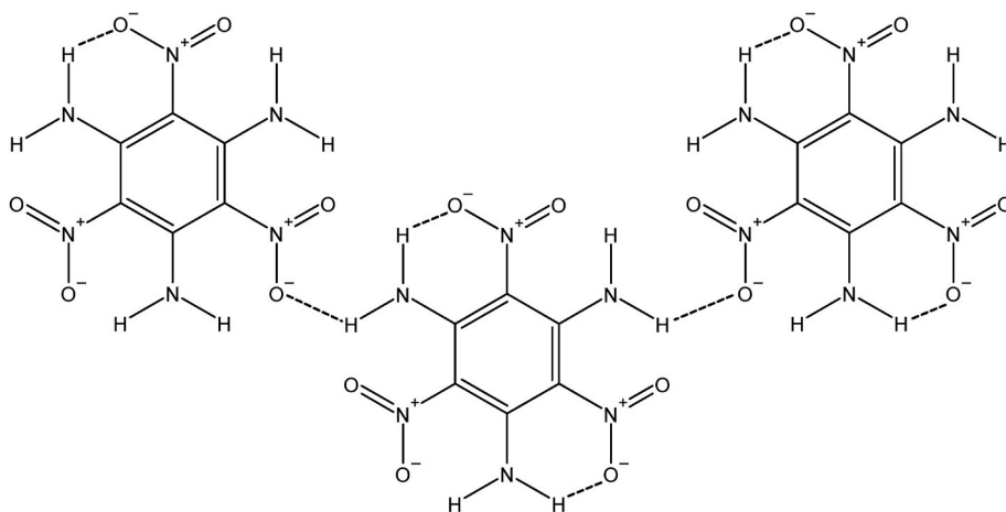
Fig. 1. Inter- and intramolecular bonding in TATB forming the graphite-like structure contributing to increasing its insensitivity to shock, thermal and impact stimuli.
