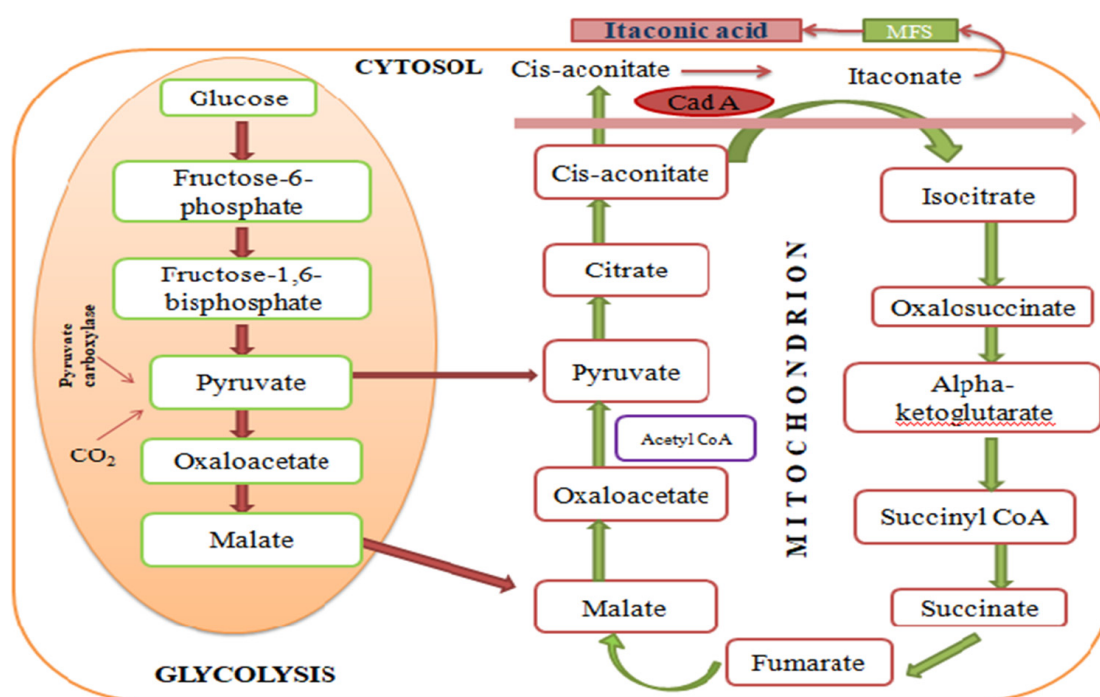
Figure 2. Biological route for IA synthesis.
