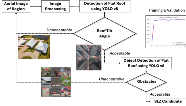
Fig. 2. System Diagram of SLZ Identification that Considers Flat Surfaces and Obstacles.
