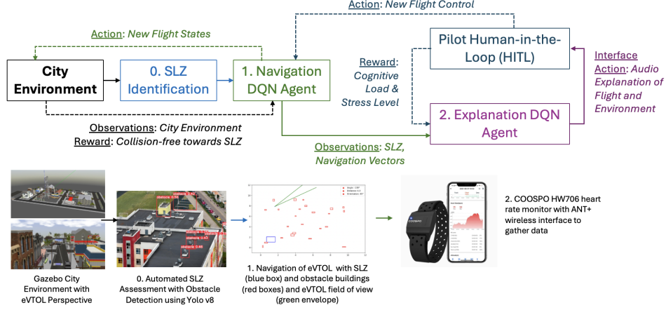
Fig. 1. System Diagram of Autonomous eVTOL Emergency Landing: 0. Safe Landing Zone (SLZ) Identification, 1. Navigation to SLZ, and 2. Cognitive Load Reduced Explanations to Pilot Human-in-the-Loop (HITL).
