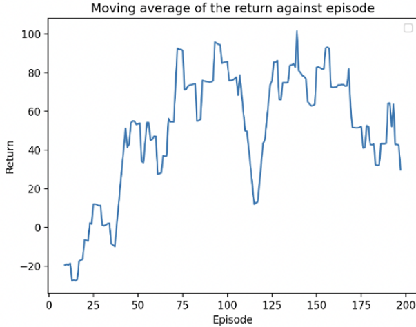
Fig. 4. 1. Navigation AC DQN RL training with learning rate hyper-parameter tuning ( \alpha_a = 10^{-5} , \alpha_c = 10^{-6} ). 2. Cognitive interface RL training with \epsilon = 0.2 .
