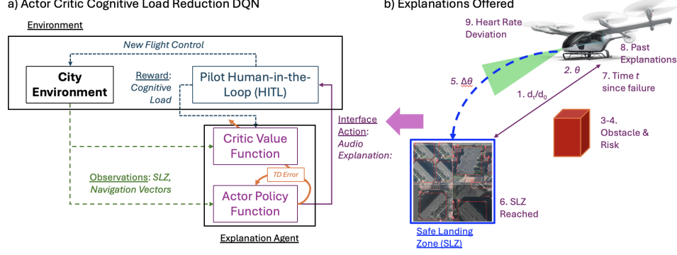
Fig. 3. a) Actor-Critic Cognitive Load Reduction DQN with Audio Explanations; b) Explanations Offered to Pilot including navigation data (1-6), eVTOL status (7), historical data (8), and heart rate deviation (9).
