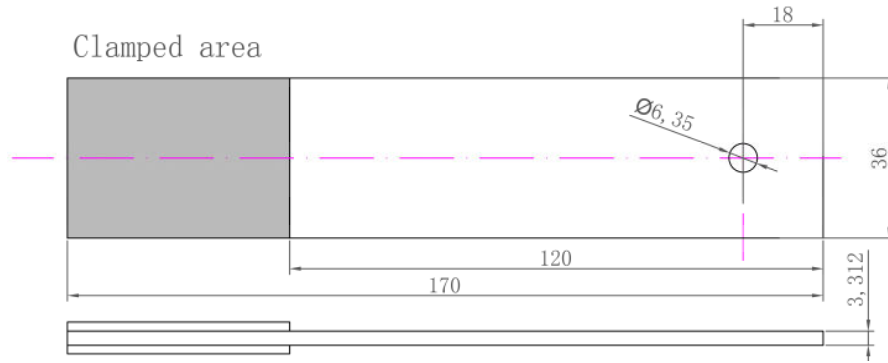
Figure 1. Dimensions of specimen
