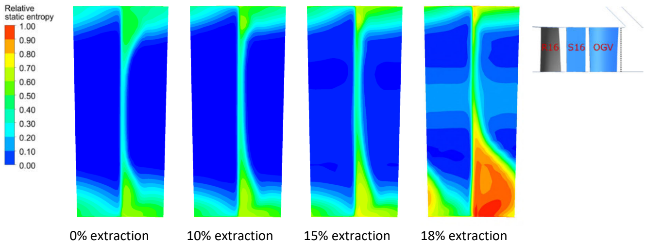
Figure 18 Static entropy contour plots behind OGV
