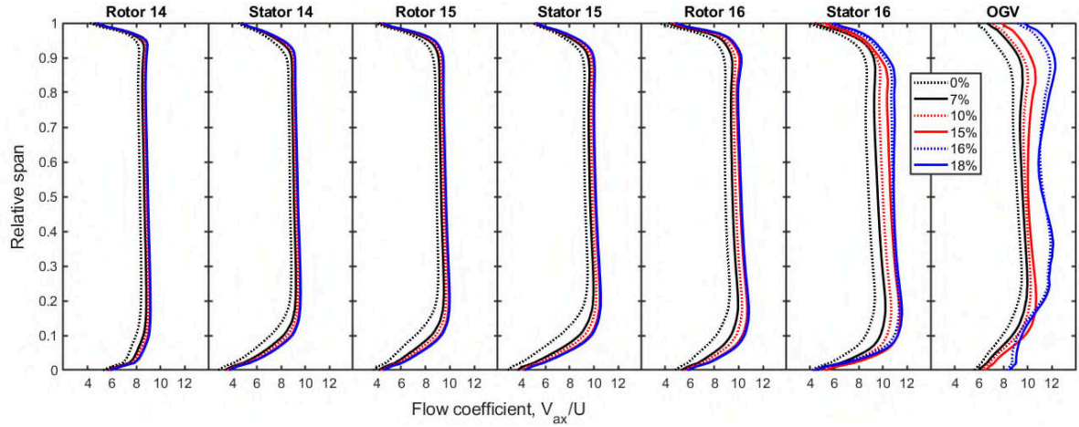
Figure 14 Stage-by-stage radial pitch-averaged flow coefficient for different extraction rates
