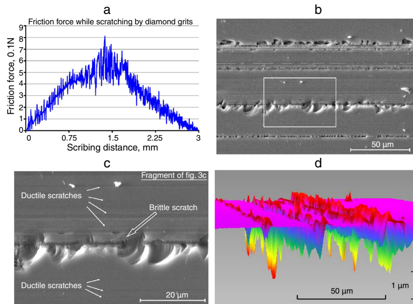
Fig. 3 – Experimental data of (a) friction force, (b) corresponding SEM images of the scratches made in silicon using arbitrarily shaped diamond particles at maximal normal load (1 N) in central part of the scratches, (c) the magnified fragment from the area (b) showing the scratches with brittle damage (in the centre) and small/very small/extremely small ductile scratches in the upper and lower part of the photo. Three-dimensional (3D) optical profilometry image (d) of the scratched area.
