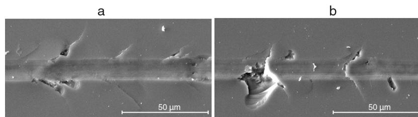
Fig. 9 – SEM images (a, b) of the central part of the scratch on silicon made using the spherically shaped single tungsten carbide grit ( \varnothing 60 \mu\text{m} ), revealing cracking and spalling.
