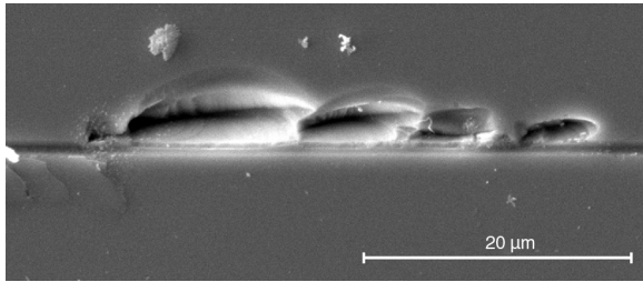
Fig. 12 – The cavities produced by the pulled-out rotating crushed tungsten carbide particle outside of the ductile scratched groove.
