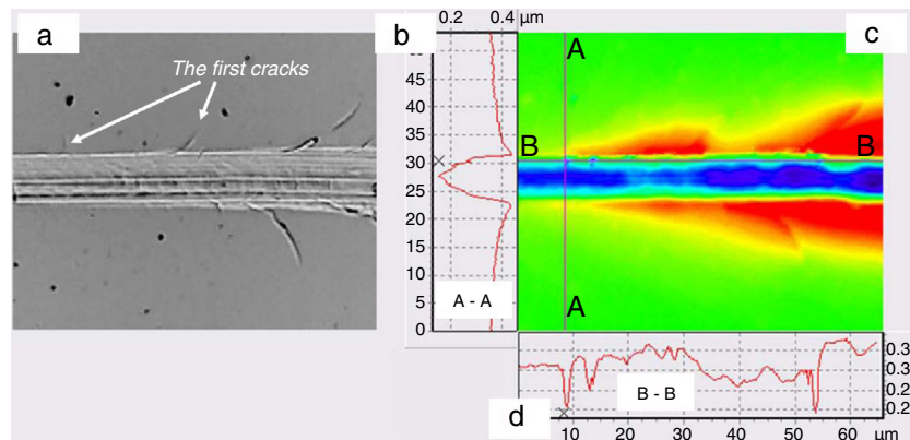
Fig. 10 – The optical image of the scratch in the area of the first cracks appearance (indicated by arrows) (a), the profile of the scratch cross-section just in the beginning of cracking (b), two-dimensional image displaying the horizontal level of lifting material by different colours (c) and longitudinal profile of the side line in the scratch (d). The vertical line A-A and horizontal line B-B in figure (c) indicate the location of the measured profile in figures (b) and (d). The area corresponds to SEM image in (c).
