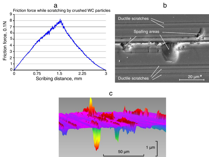
Fig. 4 – Experimental data of (a) friction force and (b) corresponding SEM image of the area scratched in silicon using crushed WC particles. 3D optical profilometry image (c) of the scratched area.
