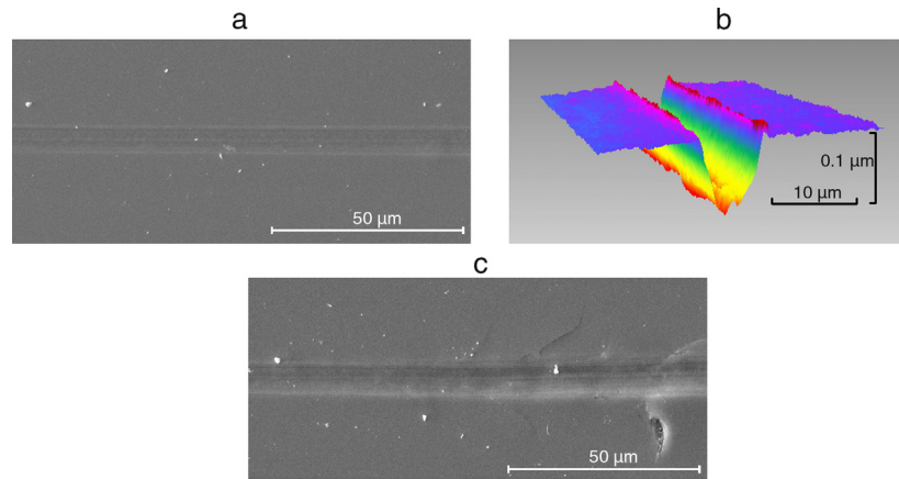
Fig. 8 – SEM image of the scratched silicon surface scribed by a single tungsten carbide grit (a) in ductile mode at the beginning of the scratch, (b) corresponding optical three-dimensional image and (c) SEM image at a scratch distance of 0.9 mm from the beginning of movement where the first cracks appeared.
