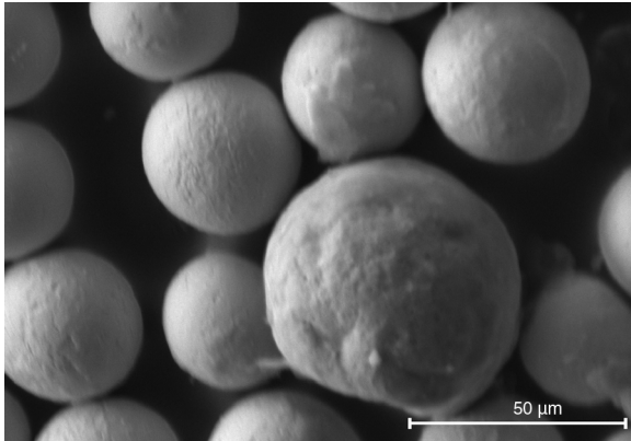
Fig. 6 – Post-SEM image of the spherical tungsten carbide particles (largest particle has 60 \mu\text{m} in diameter, which produced single scratch on the silicon plate).
