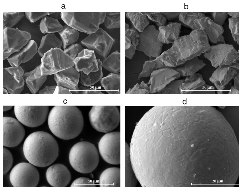
Fig. 2 – SEM images of (a) abrasive diamond particles, (b) crushed tungsten carbide particles, (c) spherical tungsten carbide particles and (d) higher magnification image of the single WC particle.
