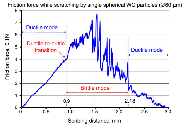
Fig. 7 – Variation in the friction force while scratching with a single tungsten carbide spherical particle ( \varnothing 60 \mu\text{m} ).
