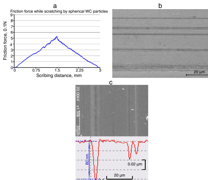
Fig. 5 – Experimental data of (a) friction force, (b) the SEM image of the area scratched in silicon using spherically shaped WC particles and (c) the SEM fragment with a few scratches and corresponding two-dimensional profile.
