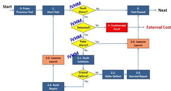
Figure 6 Test Logic of Ship Testing
