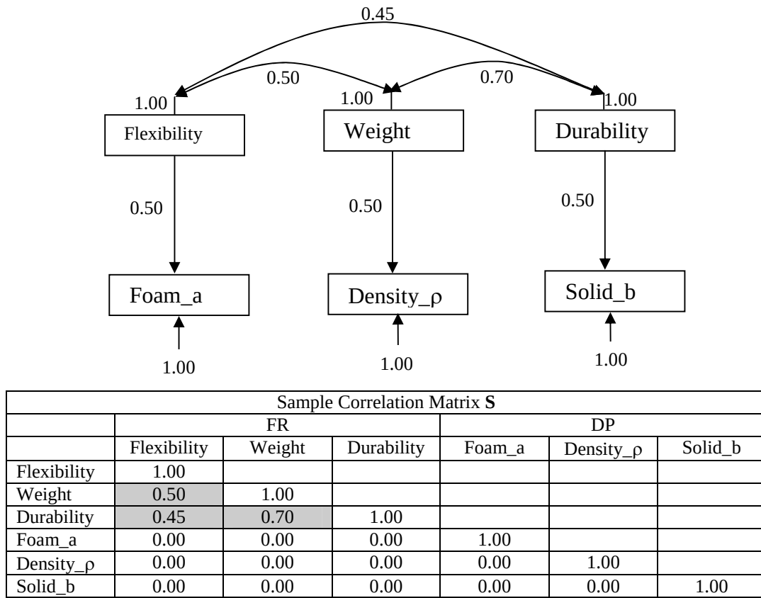
Figure 7. Structural Equation Model constructed for the injection moulding machine example.
