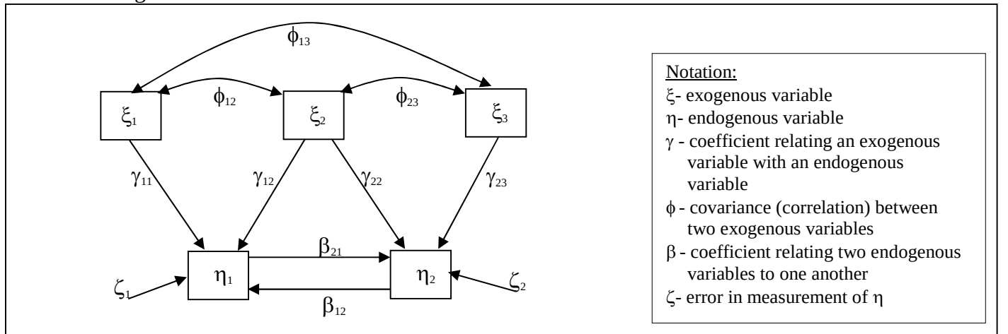
Figure 4. A structural equation model.
