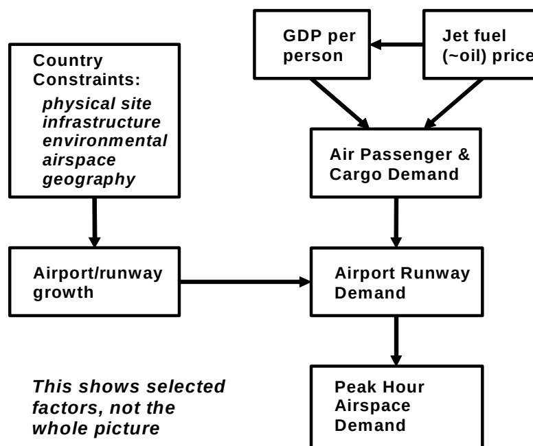
Figure 10. Selected Factors in Predicting Peak Hour Airspace Demand
