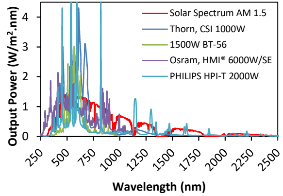
(b) Metal halide lamp [39,118,167]
