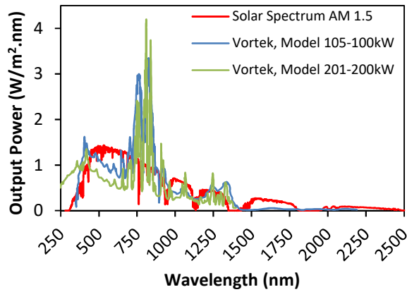
(a) Argon arc lamp [109,110]
