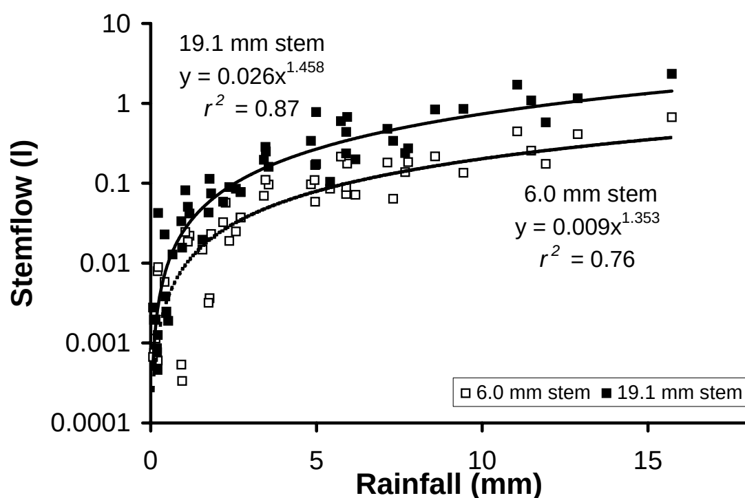
Figure 1 .The relationship between stemflow and rainfall for two willow stems of different diameter. For the 13 stems, stemflow values predicted by calculating values for a and e from equations 5 and 6 and inserting these in equation 4 accounted for 85% of the variation in actual stemflow values. The same procedure was used to estimate stemflow for all stems on all experimental plants.
