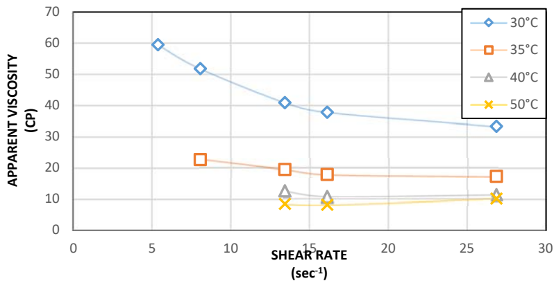
Figure 4: Effect of temperature variations on the viscosity at fixed wax concentration (37.5% wax in oil).
