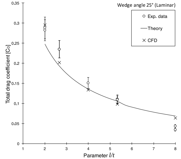
Fig 10: Comparison of experimentally measured variation of drag coefficient with l/t , with theory and CFD. \delta = 25^\circ , Laminar interaction.
