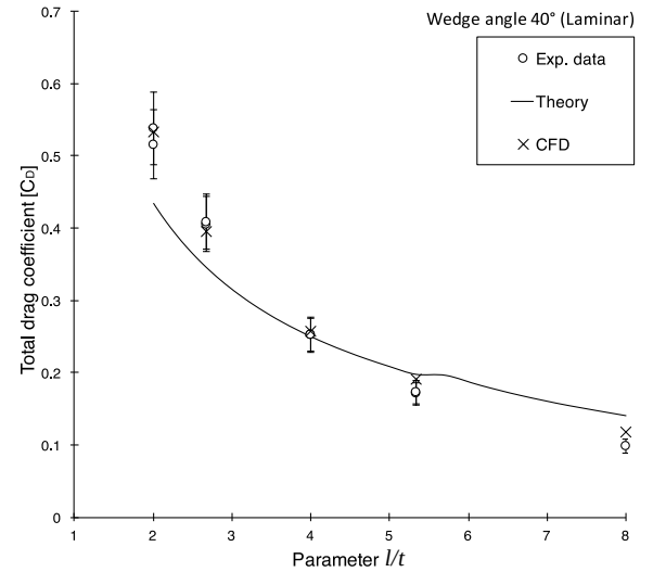
Fig 11: Comparison of experimentally measured variation of drag coefficient with l/t , with theory and CFD. \delta = 40^\circ , Laminar interaction.
