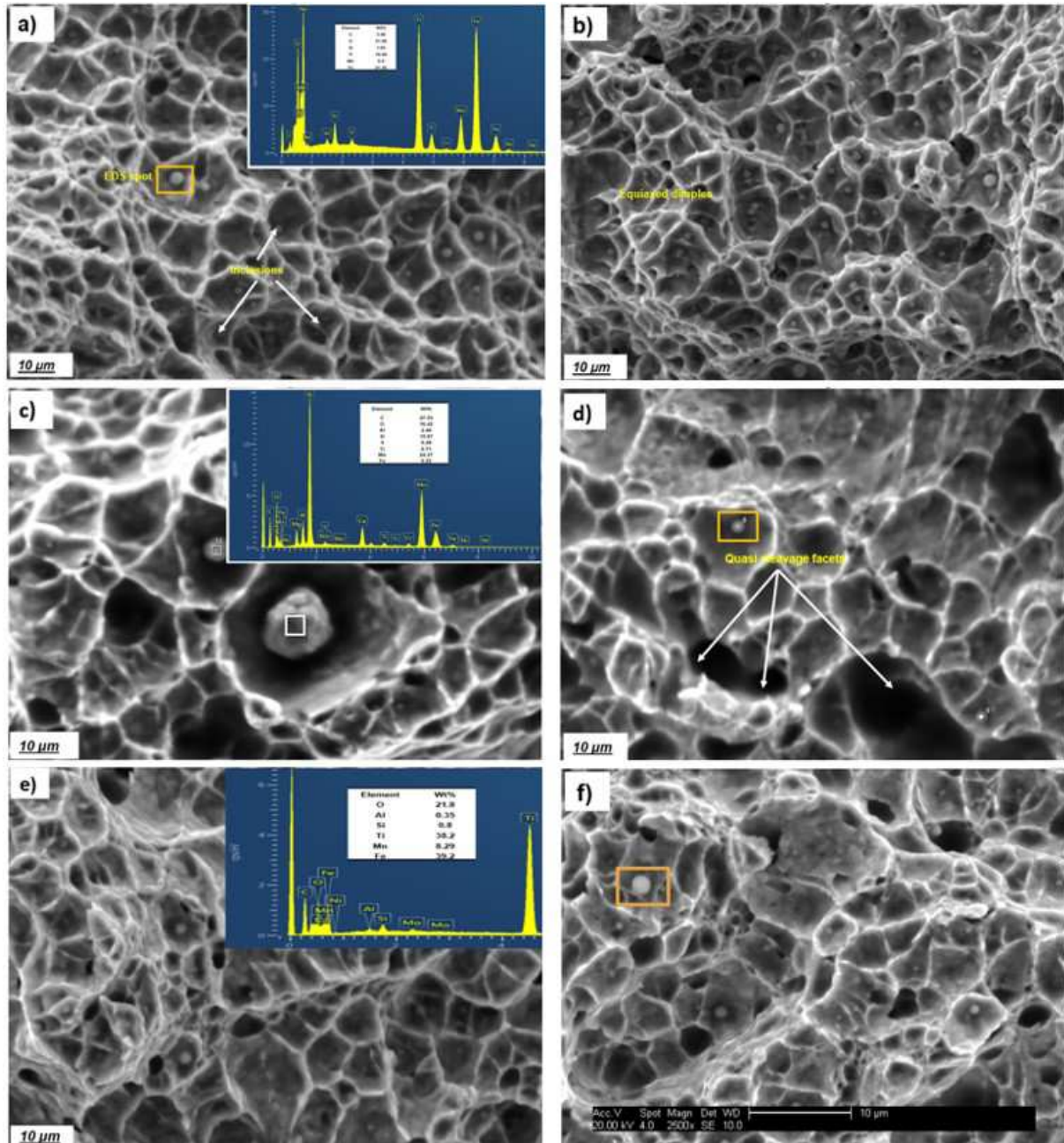
Fig. 14 : Fracture morphologies for J1C specimen in both X & Z direction with EDS analysis of round particles (a) ER70S-6(Z) (b) ER70S-6(X) (c) 90S-B(Z) (d) 90S-B (X) (e) ER120S-G (Z) (f) ER120S-G (X)
