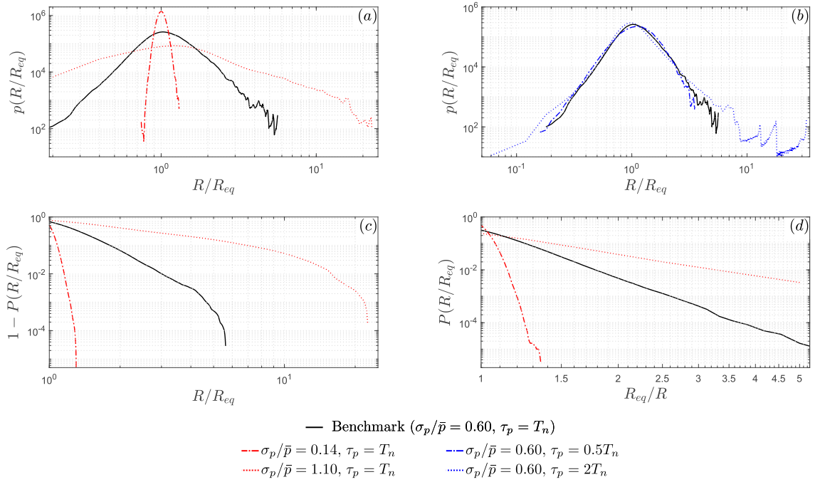
FIG. 8. (a, b) Probability density function of the metric R/R_{eq} . (c) Complementary cumulative distribution function of R/R_{eq} evaluated for R/R_{eq} > 1 (right tail of the distribution). (d) Cumulative distribution function of R/R_{eq} evaluated for R/R_{eq} < 1 (left tail of the distribution), note that the horizontal axis reports R_{eq}/R and not R/R_{eq} as in Panel (c).
