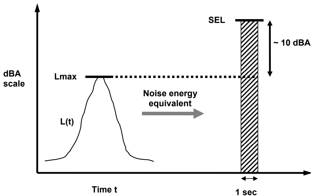
Figure 3. Noise definitions
