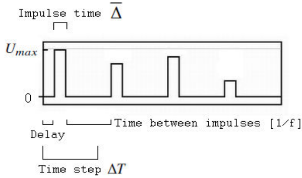
Fig. 4 Representation of a pulse-amplitude modulation strategy of generating thrust on a specific LVLH direction.
