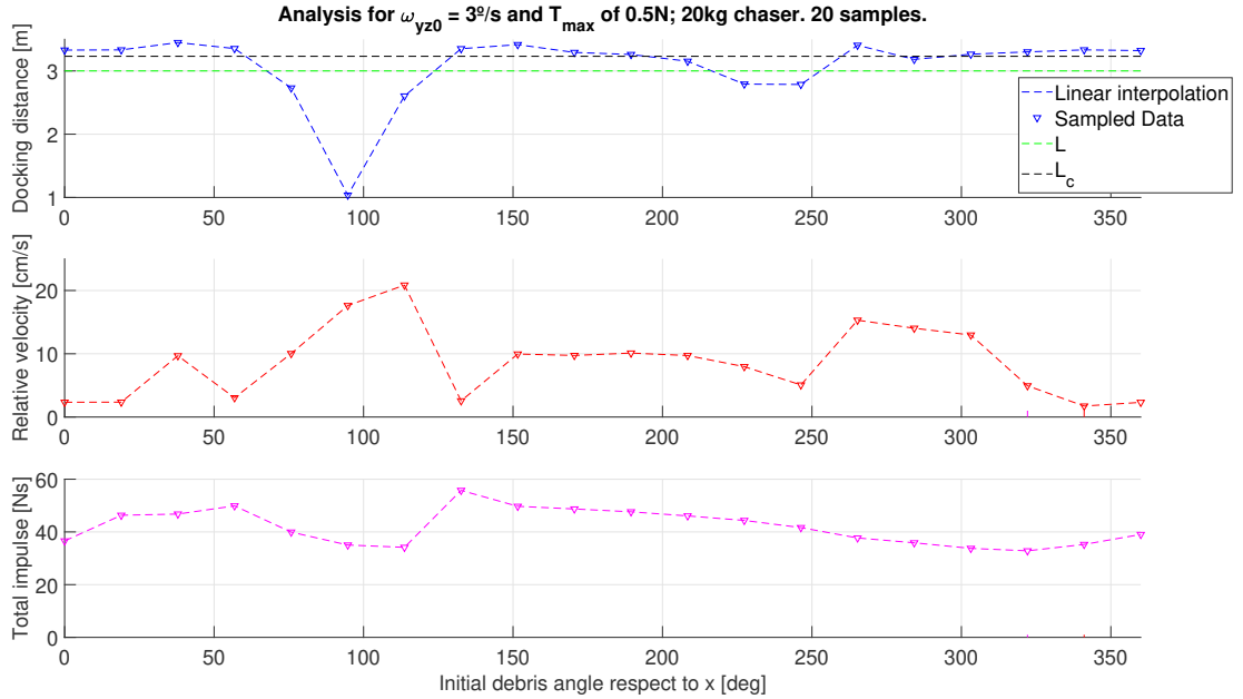
Fig. 15 Docking distance, relative velocity at docking, and Total Impulse with the initial relative attitude for U_{\max} = 0.5 N, \omega_{yz0} = 3 deg/s.
