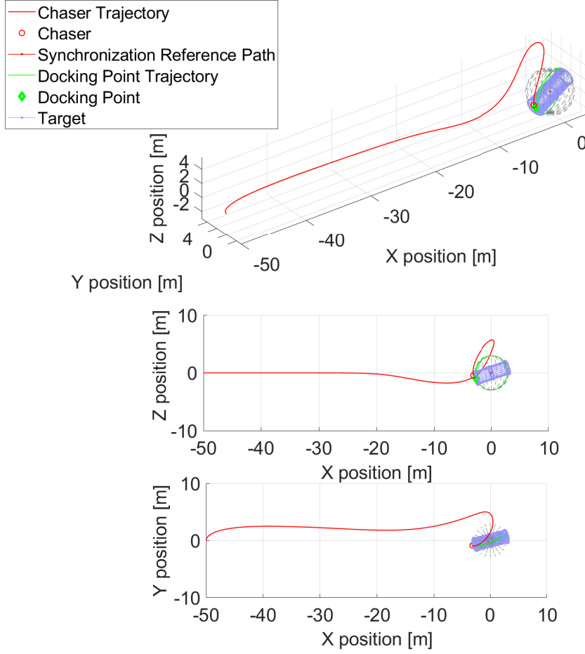
Fig. 11 Trajectory followed by the chaser for the case with U_{\max} = 500 mN, \omega_{yz0} = 3 deg/s, perturbations, and noise in navigation inputs.
